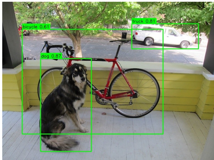
Figure 6: YOLOv4-tiny correctly detecting dog (0.87), truck (0.81), and bicycle (0.61) in a reference image.
