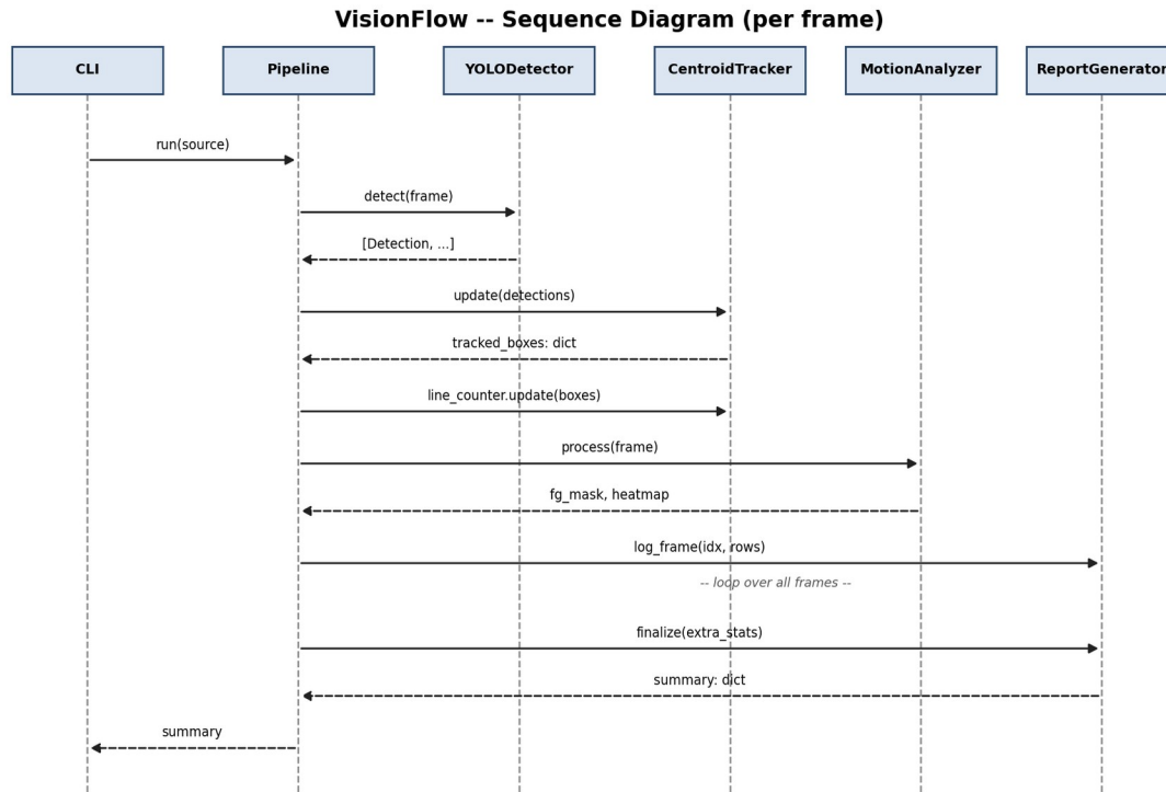
Figure 4: Per-frame sequence of calls between the Pipeline and its collaborators.
