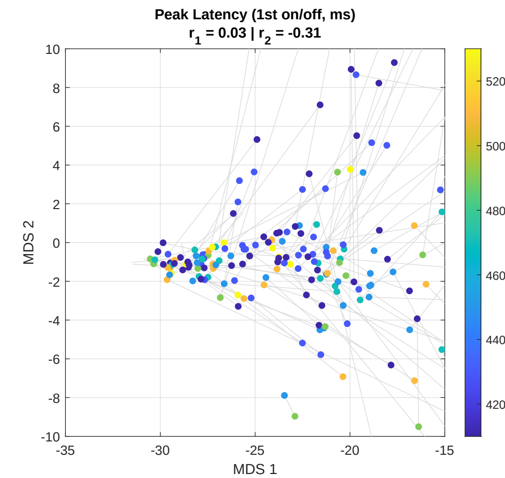
Joint MDS colored by raster/PSTH features (zoomed)
