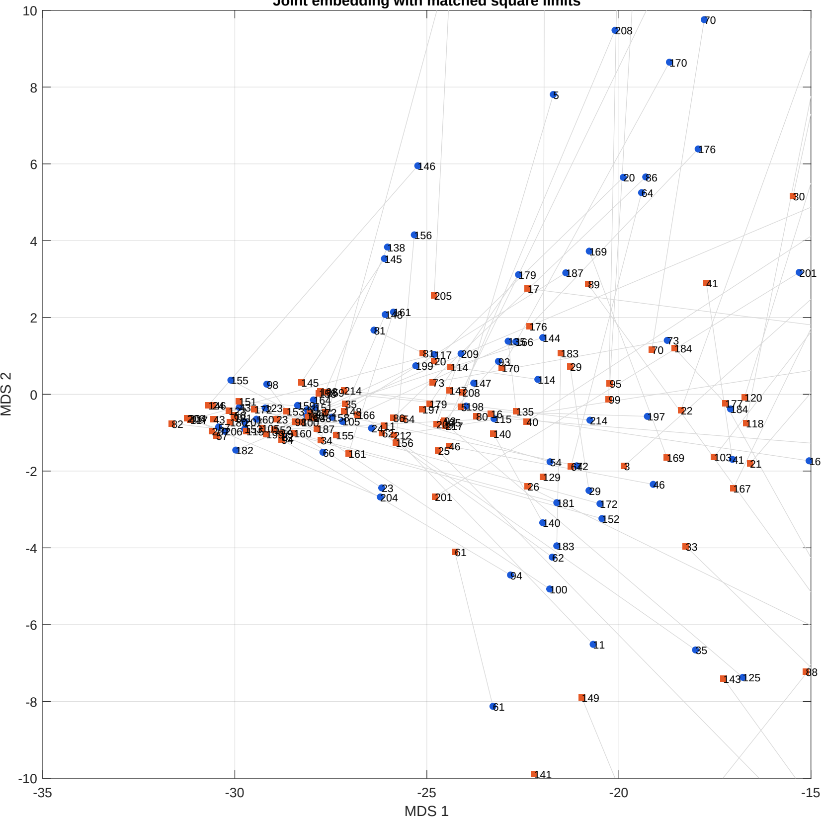
Joint embedding with matched square limits
