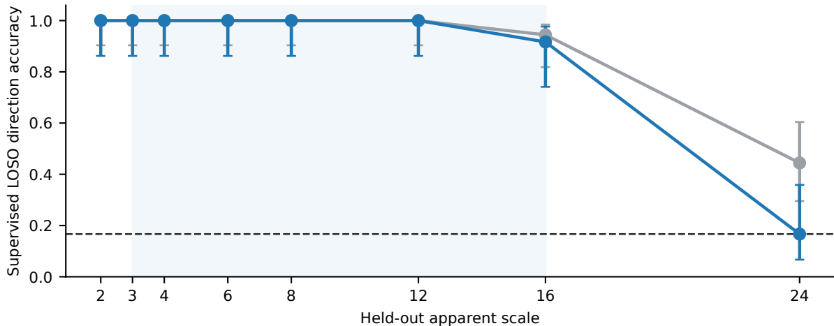
Strong interior transfer, chance performance at the upper boundary
