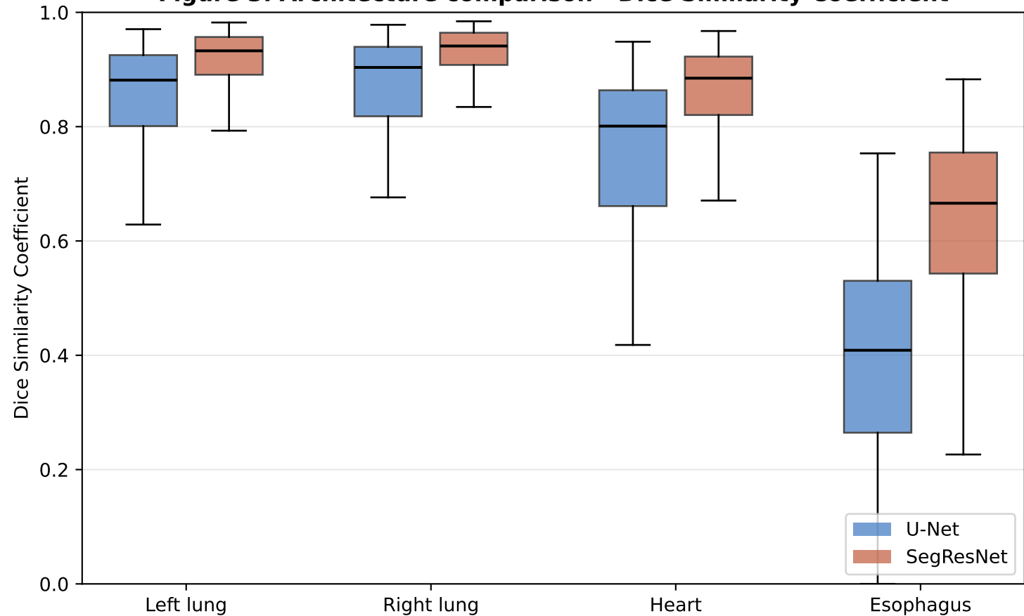
Figure 3. Architecture comparison - Dice Similarity Coefficient
