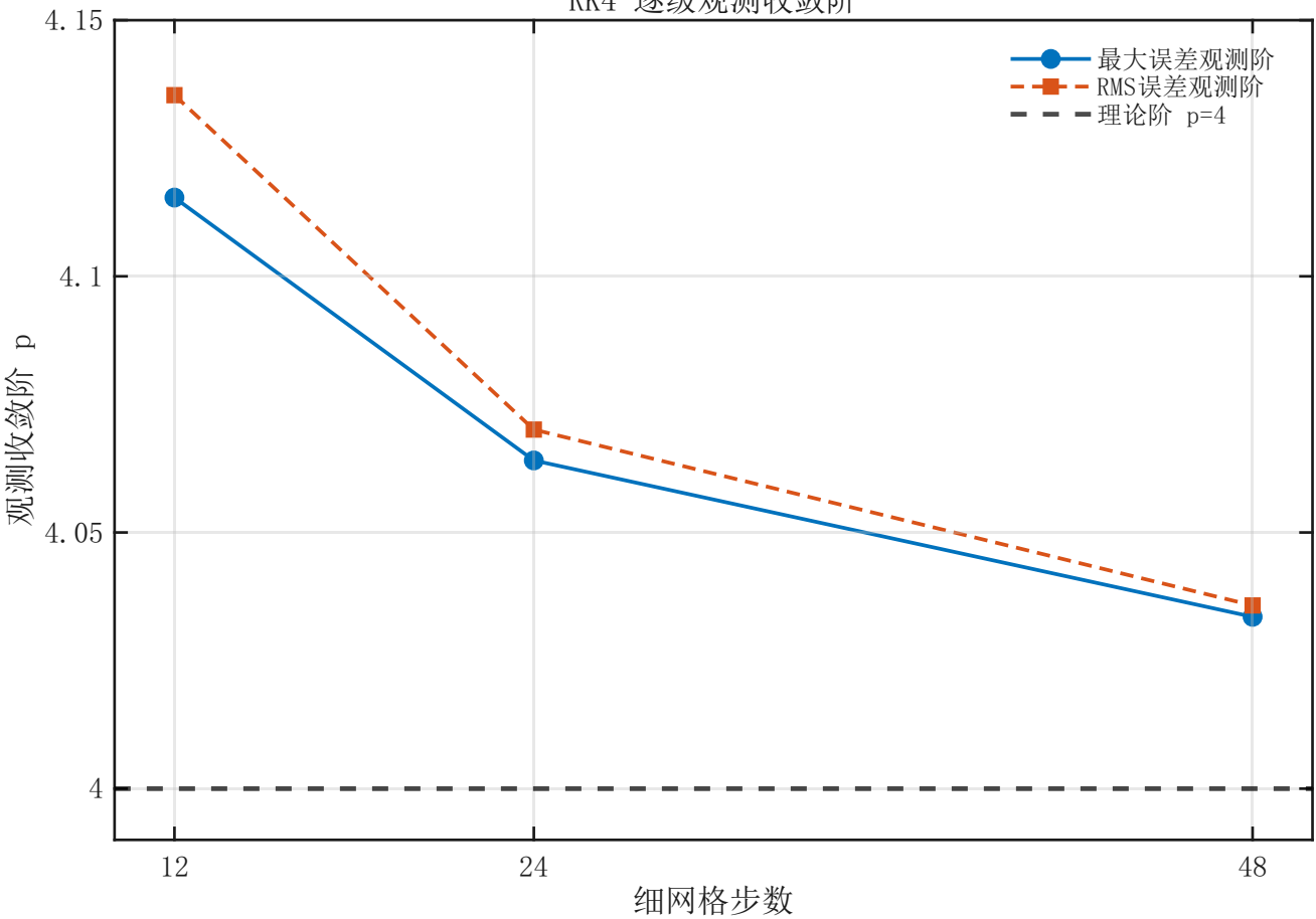
RK4 逐级观测收敛阶
