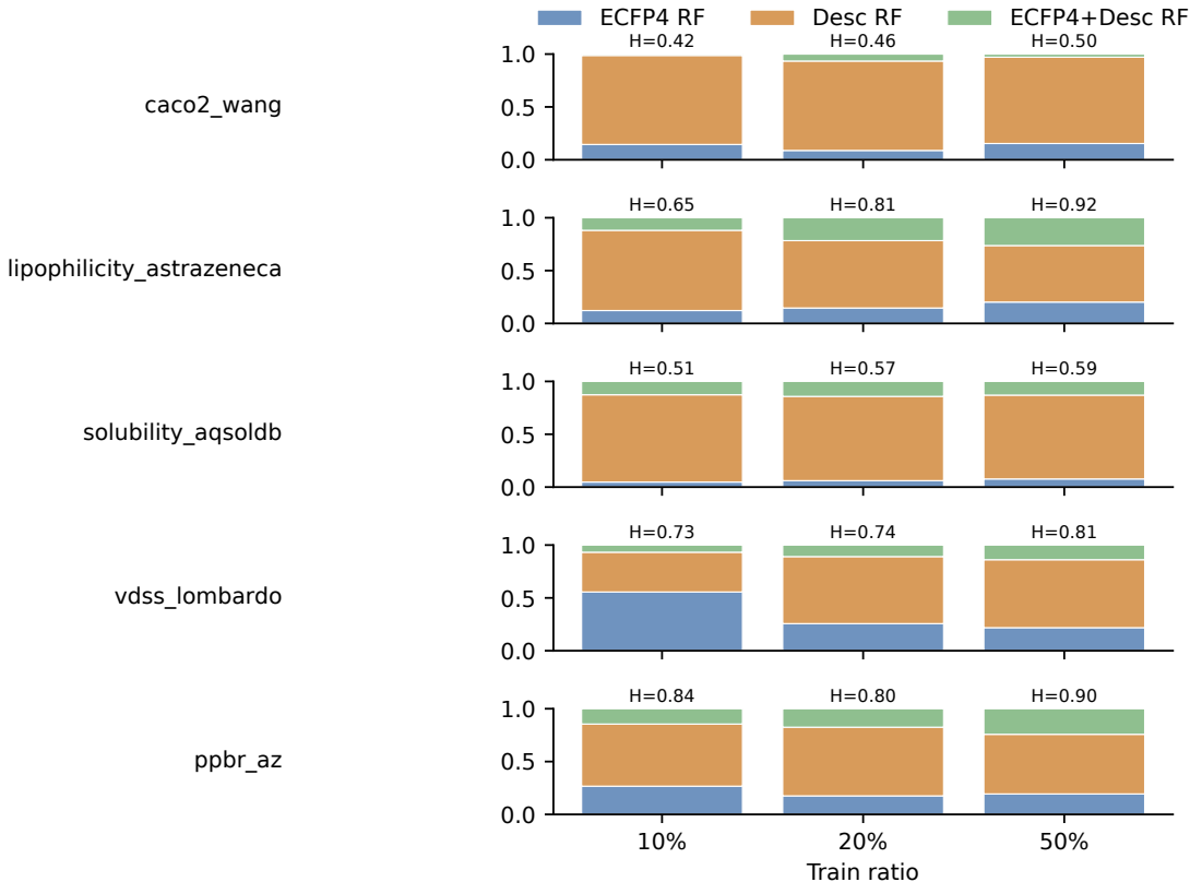
Figure 4: Selector routing choices by endpoint and train ratio. Bars show the test-split proportion of samples routed to each RF teacher, averaged across three seeds. H denotes normalized entropy of the routing distribution.
