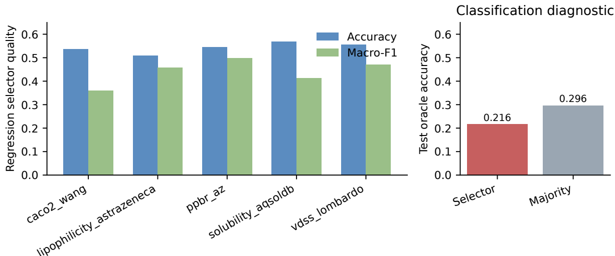
Figure 5: Selector quality diagnostics. Left: regression selector accuracy and macro-F1 by endpoint. Right: the same selector protocol fails on classification diagnostics, where test oracle-teacher accuracy is below the train-majority baseline.
