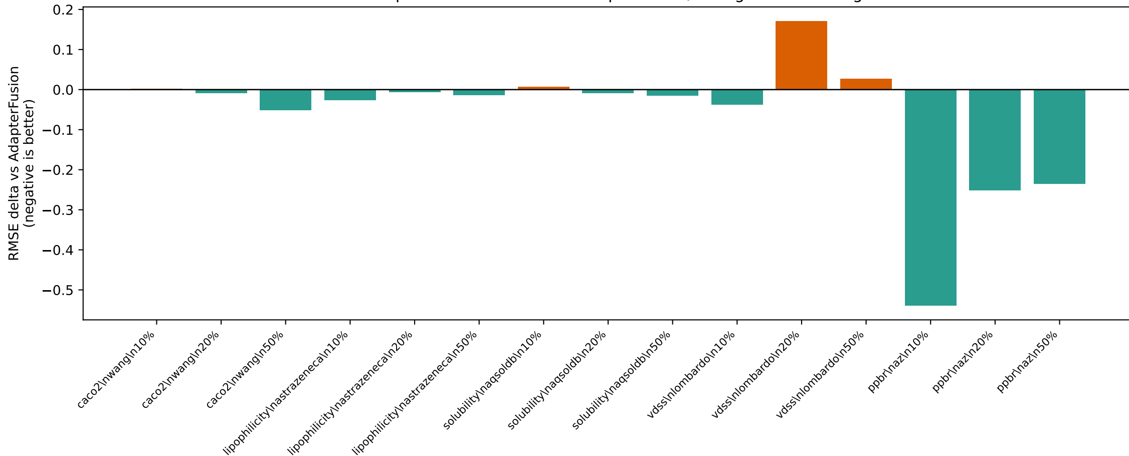
Descriptor-teacher distillation improves 11/15 regression settings
