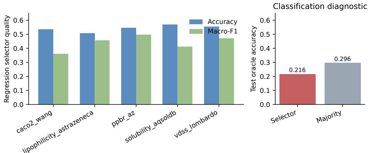
Figure 4: Selector quality diagnostics. Left: regression selector accuracy and macro-F1 by endpoint. Right: the same selector protocol fails on classification diagnostics, where test oracle-teacher accuracy is below the train-majority baseline.
