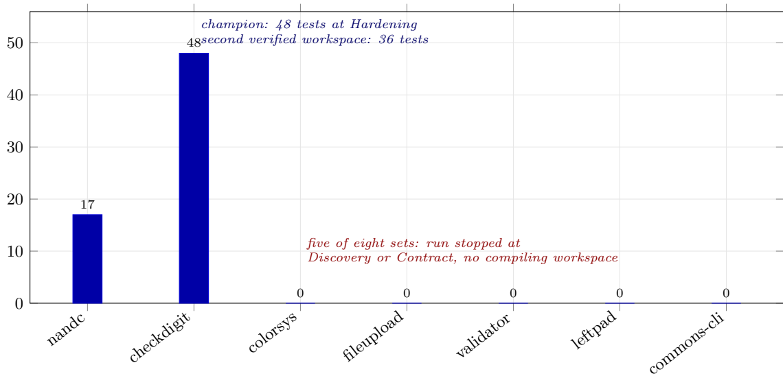
Toolchain-verified tests passed
