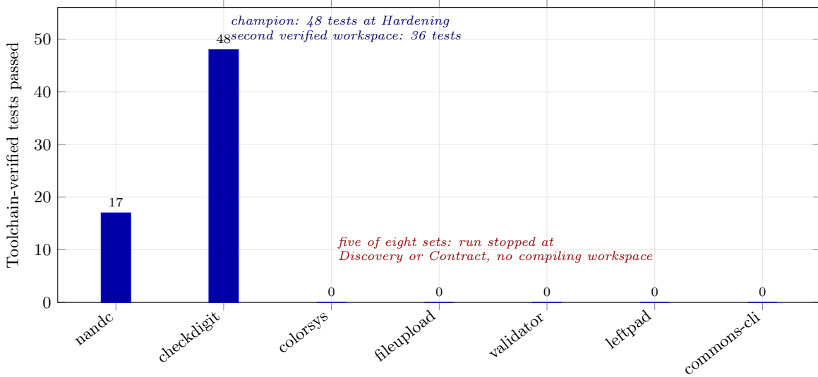
Figure 3: Cleared problems per dataset family at the 2026-10-04 scoreboard (13 of the brief’s 114). The figure preserves the earlier four-day search campaign’s per-set test peaks (nandc 17, checkdigit 48 and 36); the sweep-phase cleared problems are counted once per problem, across retries, from the per-round ledger.
