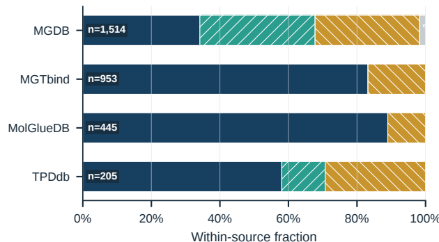
b Relation composition by source
