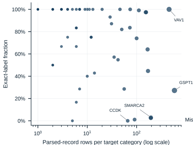
c Exact-label fraction across target categories
