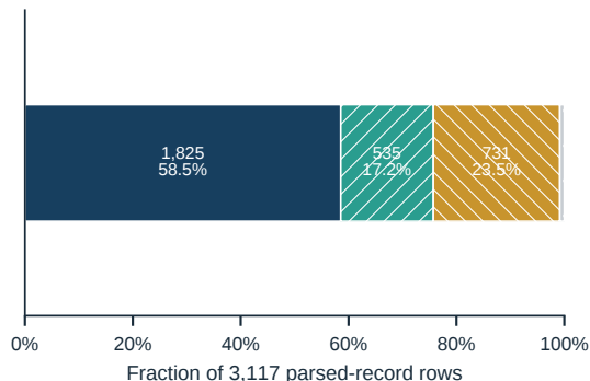
a Parsed DC50 record-table rows
