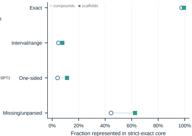
d Structure overlap with strict-exact core
