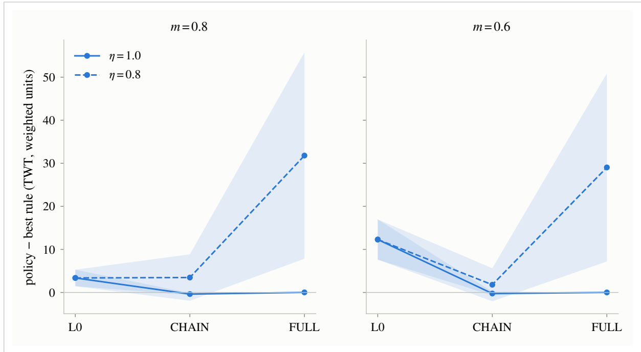
Figure S4. The flexibility gradient: policy-versus-best-ranked-rule TWT gap (seed mean, per-seed ribbon) as a function of structure, panels = crew multiplier, both \eta values. Positive gap means the policy is worse. The ribbon shows training-seed variability only; workload uncertainty is carried separately by the per-cell bootstrap intervals in the released tables. Policy numbers are 10-seed means; n per cell in the released tables. Gate P outcome: did not pass (branch B). Takeaway: the policy-versus-rule gap narrows on the chain and reverses in the chained cells at \eta = 1 , but re-opens under full flexibility once the efficiency penalty bites.
