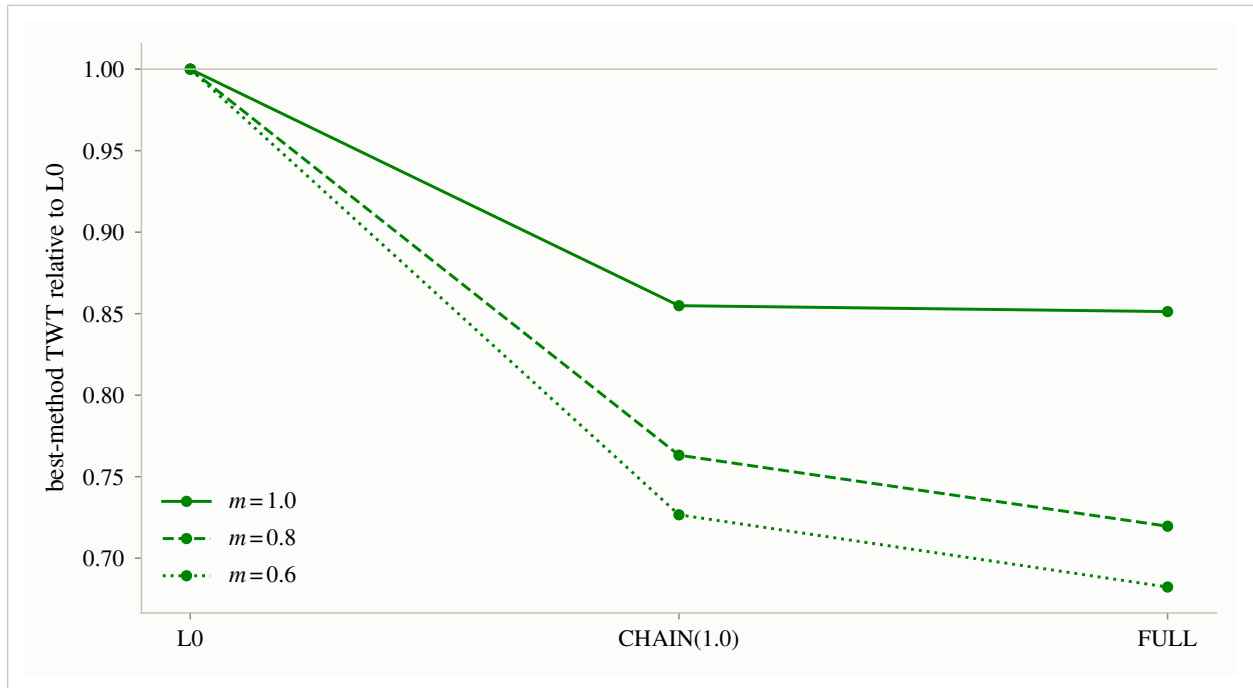
Figure S6. Stress test on the deliberately under-provisioned held-out campus 2: best-method TWT relative to the dedicated baseline across structures, \eta = 0.8 , three crew multipliers; n per cell in the released tables. Intervals are instance-level only, because the result comes from one campus. Takeaway: on this stress-test campus the simulation values cross-training at up to 32% lower weighted tardiness (complete chain 27%), so flexibility hedges a crew mis-calibration where it hurts most.
