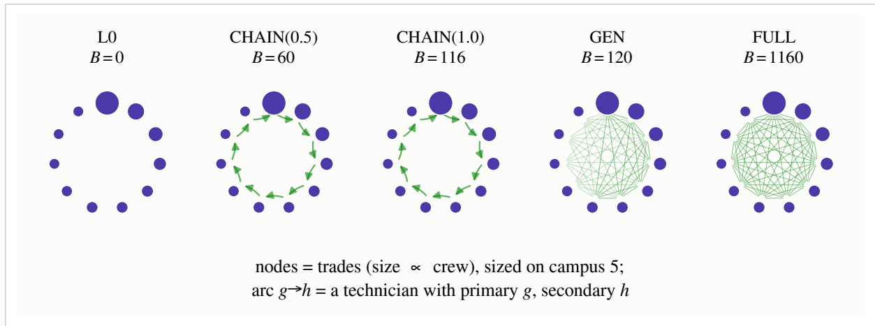
Figure S3. The flexibility ladder on one real campus, as trade-level eligibility structure: nodes are trades on a circle in chain order (size proportional to crew), and a directed arc g \rightarrow h marks a technician with primary trade g and secondary skill h . L0 has no arcs; CHAIN(1.0) is a single directed cycle covering all trades; GEN is a hub of generalists; FULL is complete (the dense GEN and FULL meshes are drawn as headless chords for legibility). The realized skill-membership budget B is annotated; headcount is identical in every panel. Takeaway: the ladder spans dedicated to fully flexible at fixed headcount, with the complete 2-chain a single cycle that grants one secondary skill per technician.
