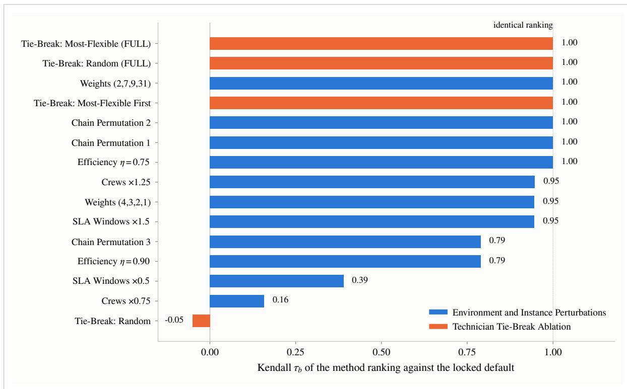
Figure S2. Robustness of the method ranking: Kendall \tau_b between the ranking under each sensitivity variant and the locked default, designated cells, n = 120 per variant, shown as ranked bars. Takeaway: rankings survive the efficiency, weight-vector and chain-order perturbations, move only where the perturbation forces deeper overload, and collapse when the technician tie-break is randomized.
