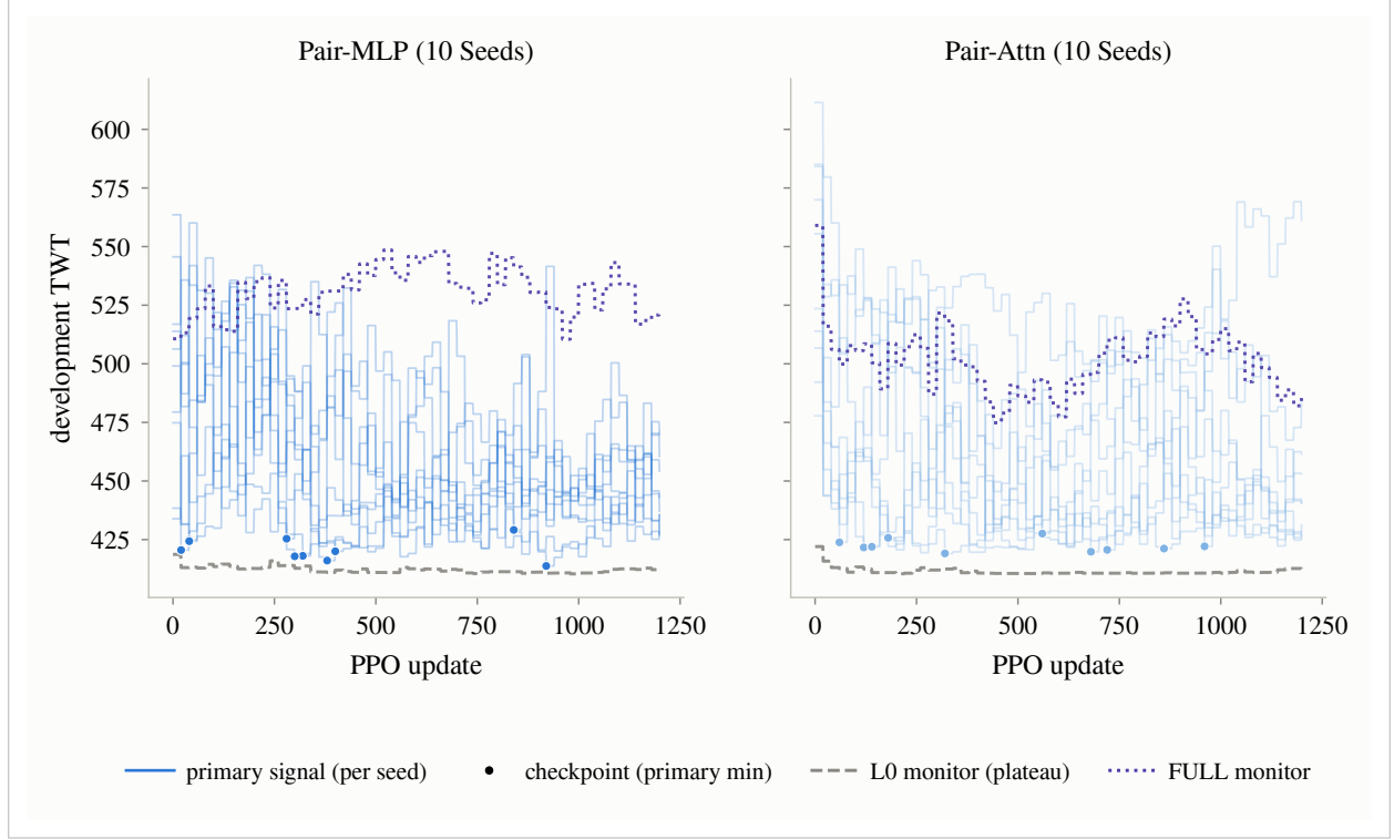
Figure S1. Training diagnostics: primary development signal (tight-capacity chain cell) and monitors per update, 10 seeds per class, checkpoint at the per-seed primary minimum. Takeaway: the tight-capacity development signal discriminates checkpoints that the default-capacity monitors cannot.
