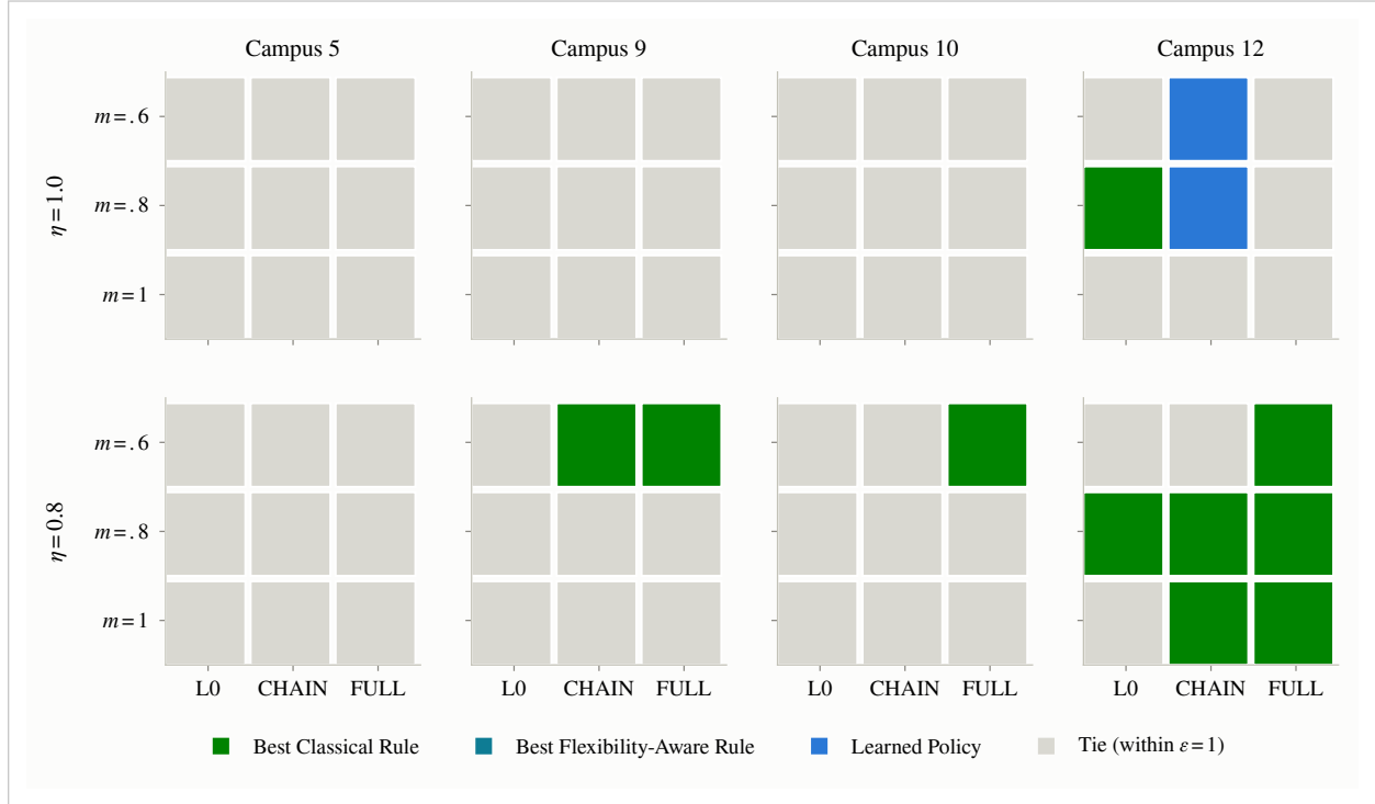
Figure S5. Decision map: cells over crew multiplier \times structure, colored by the winner among the best classical rule, the best flexibility-aware rule, and the policy (10-seed mean); one panel per verdict campus, one row per \eta , replay track. Takeaway: most cells are ties, the cells that separate go to the classical rules, and the learned policy's only outright wins are chained cells at \eta = 1 .
