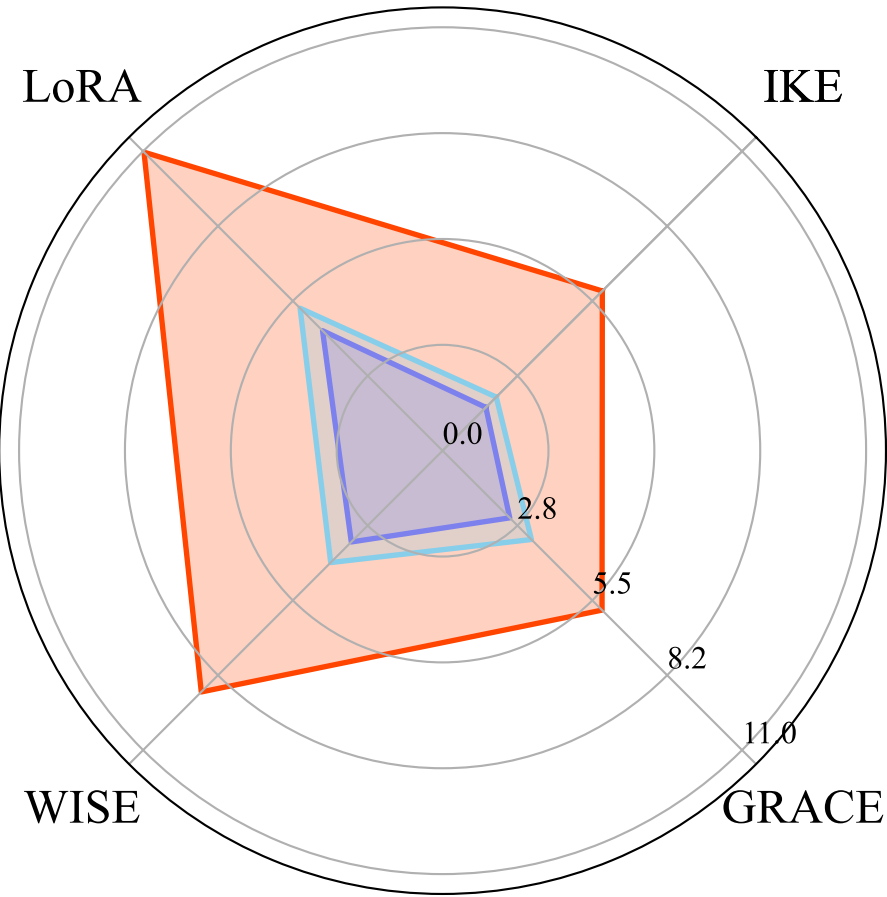
Avg Time per Sample (s) - Reasoning
