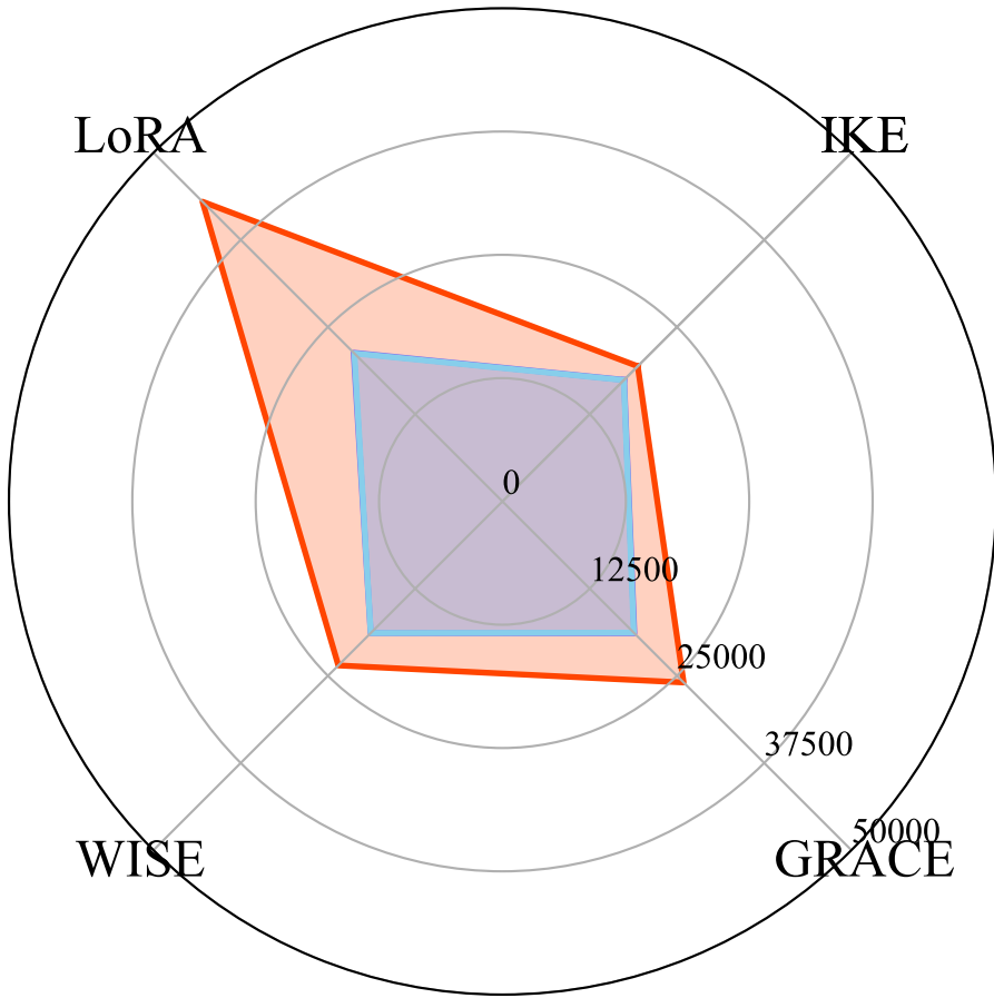
Peak GPU Memory (MB) - Reasoning
