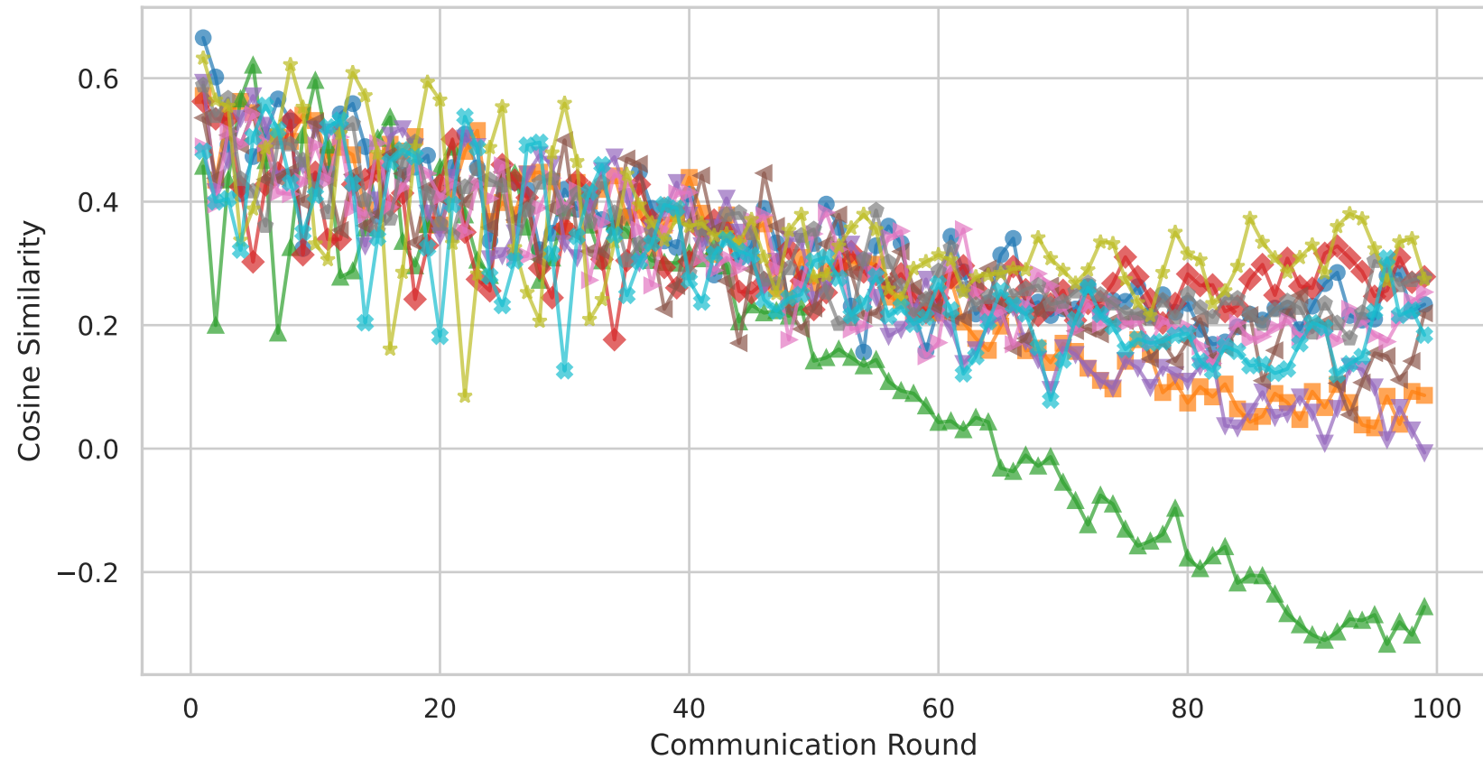
FedGTA - Client Cosine Similarity [CIFAR100 \alpha=0.01 ]
