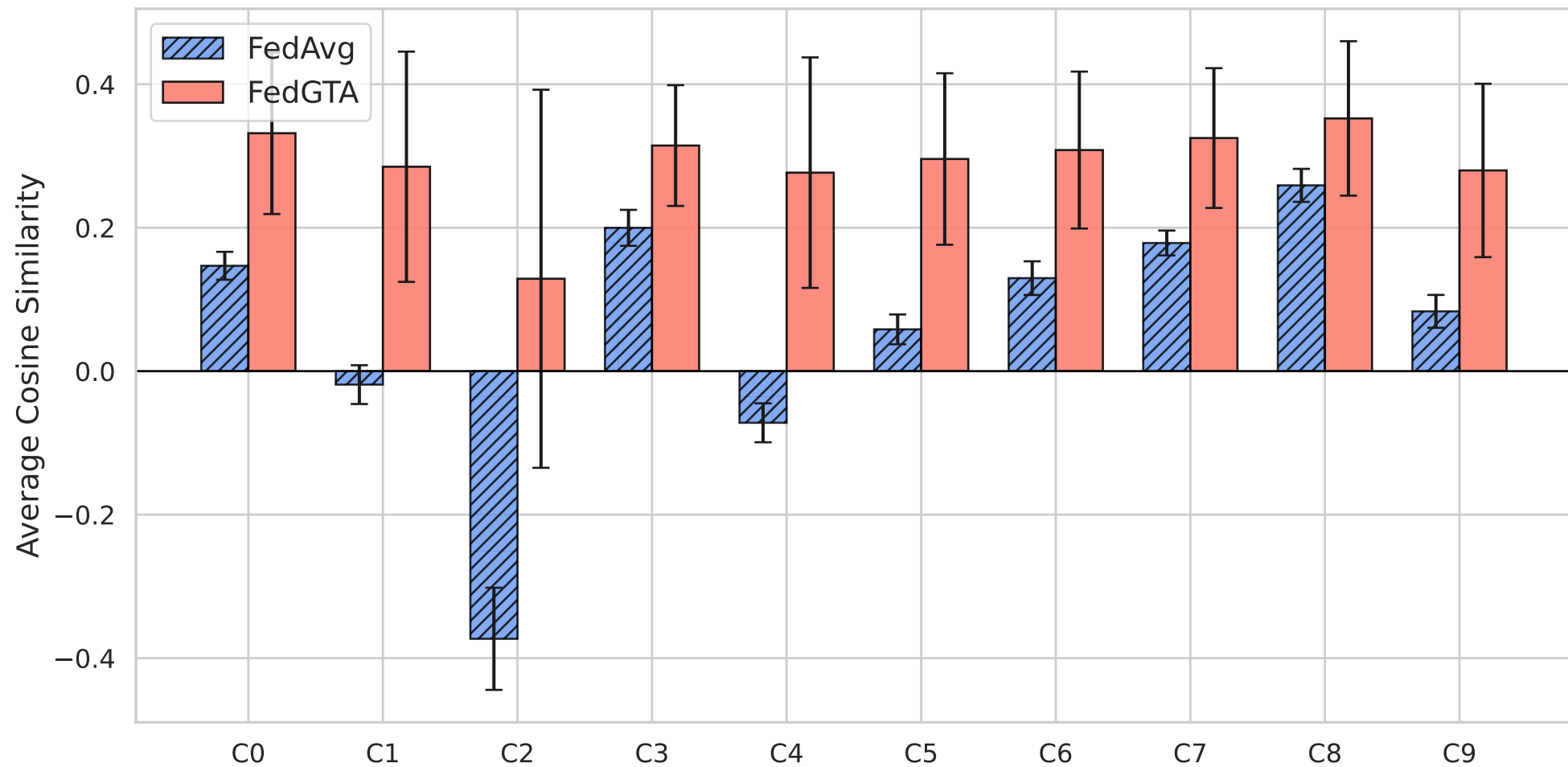
Client-wise Cosine Similarity Distribution - CIFAR100 ( \alpha=0.01 )
