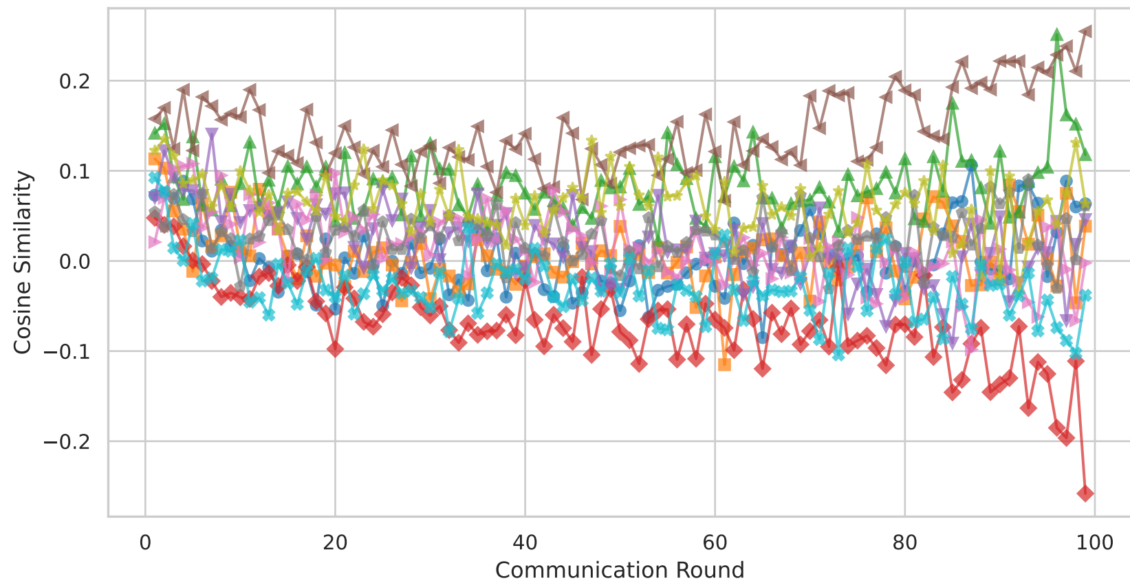
FedAvg - Client Cosine Similarity [CIFAR100 \alpha=0.1 ]
