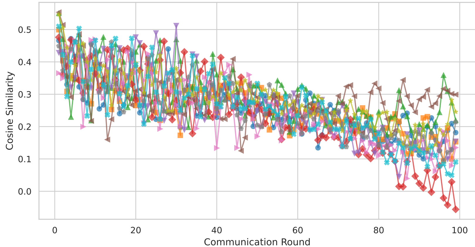
FedGTA - Client Cosine Similarity [CIFAR100 \alpha=0.1 ]
