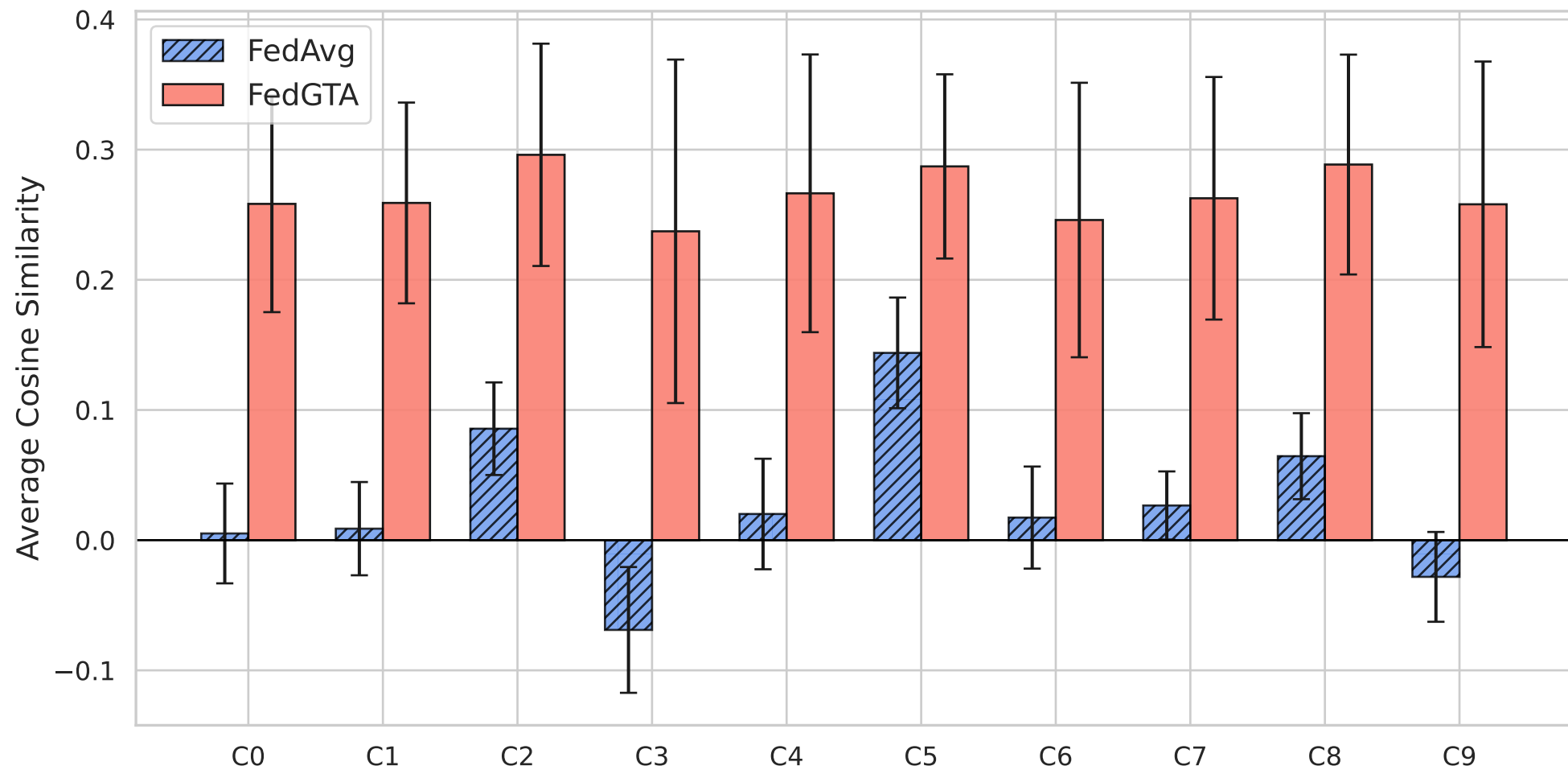
Client-wise Cosine Similarity Distribution - CIFAR100 ( \alpha=0.1 )
