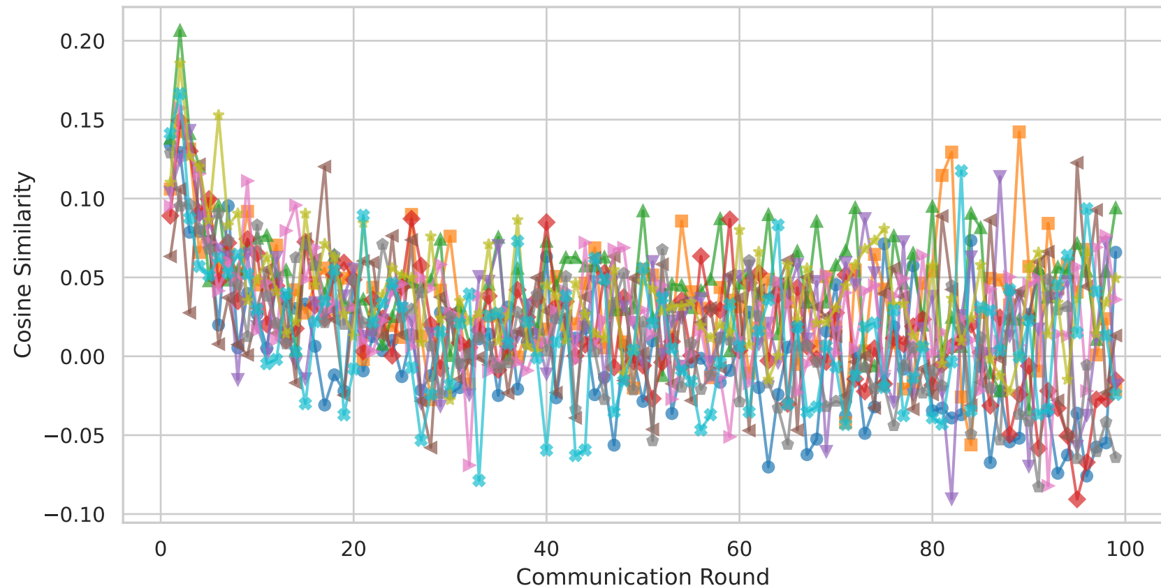
FedAvg - Client Cosine Similarity [CIFAR100 \alpha=1 ]
