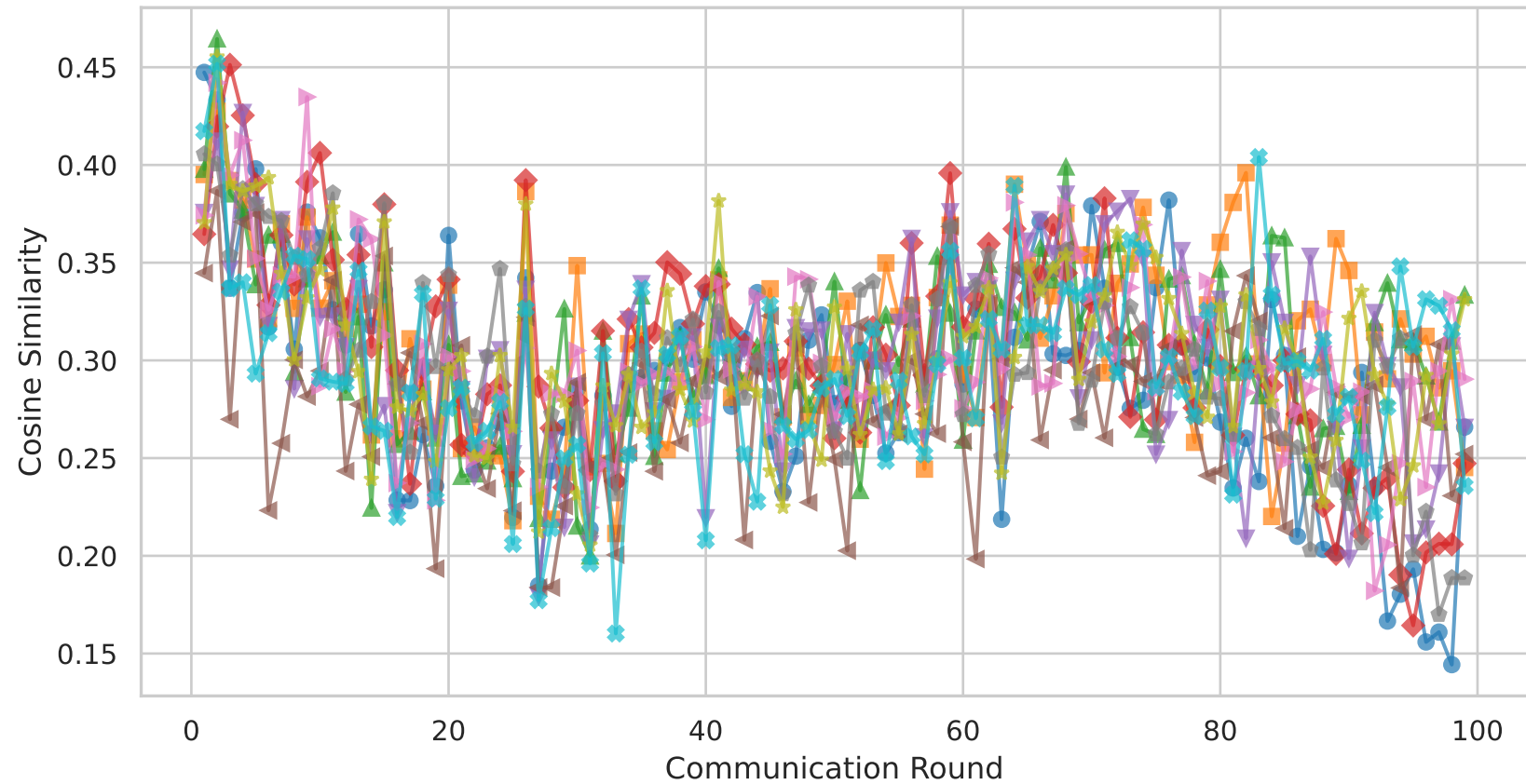
FedGTA - Client Cosine Similarity [CIFAR100 \alpha=1 ]
