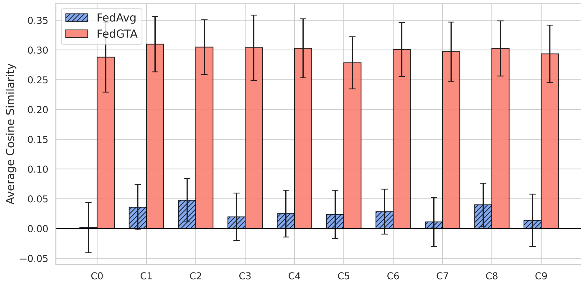
Client-wise Cosine Similarity Distribution - CIFAR100 ( \alpha=1 )
