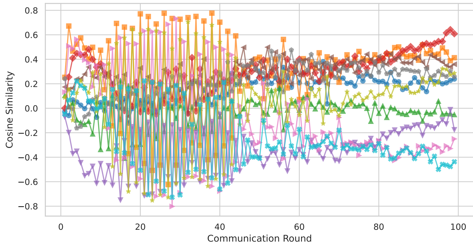
FedAvg - Client Cosine Similarity [FashionMNIST \alpha=0.01 ]
