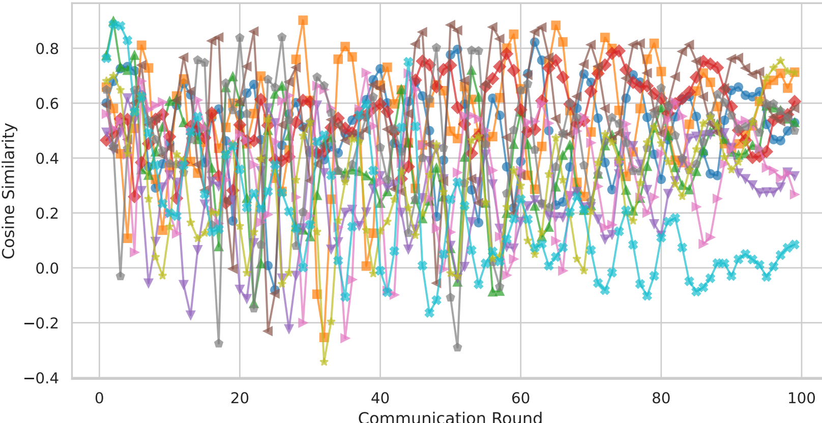
FedGTA - Client Cosine Similarity [FashionMNIST \alpha=0.01 ]
