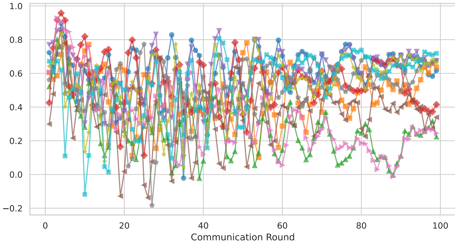
FedGTA - Client Cosine Similarity [FashionMNIST \alpha=0.1 ]
