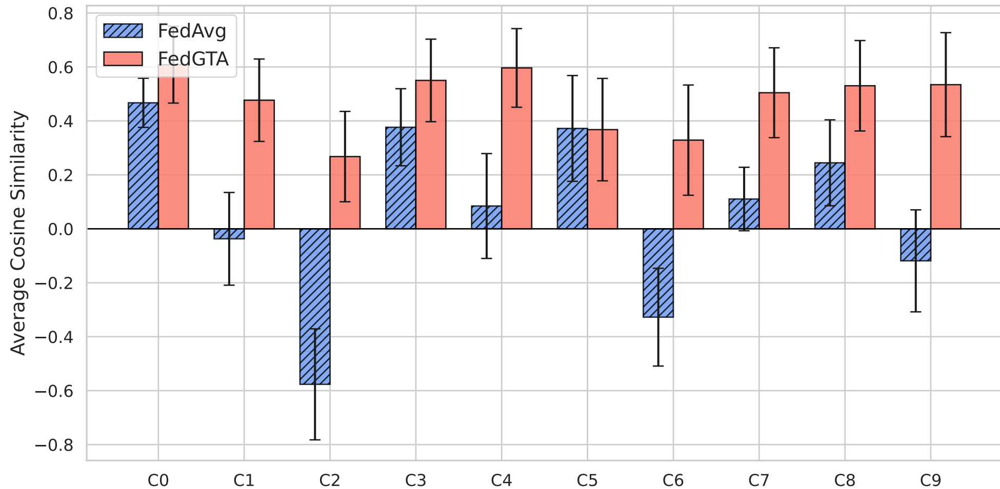
Client-wise Cosine Similarity Distribution - FashionMNIST ( \alpha=0.1 )
