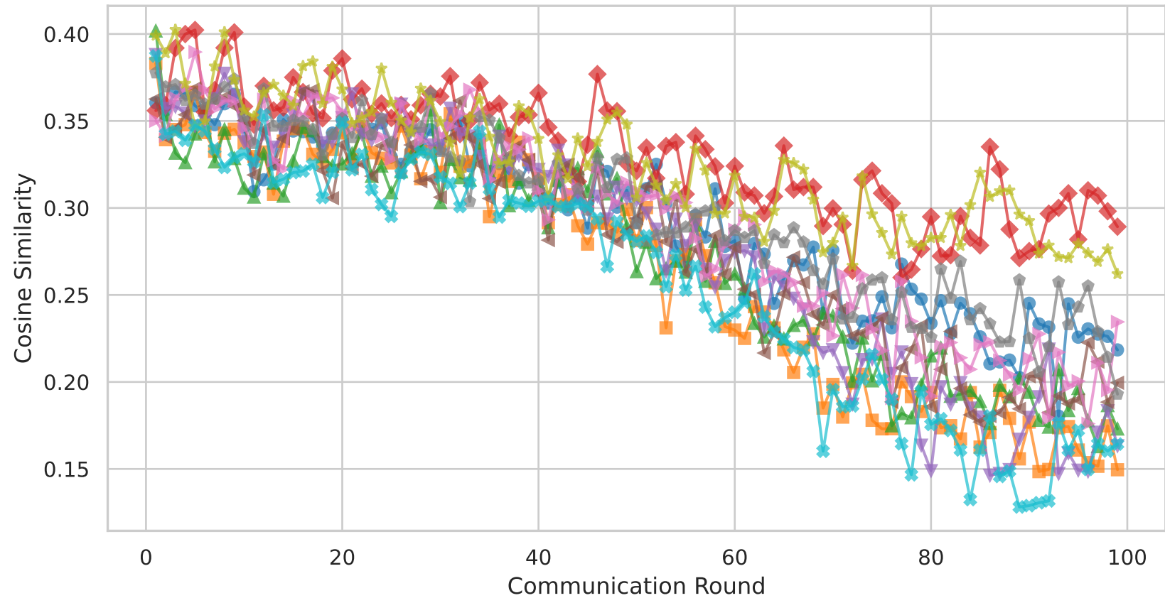
FedGTA - Client Cosine Similarity [ImageNet \alpha=0.01 ]
