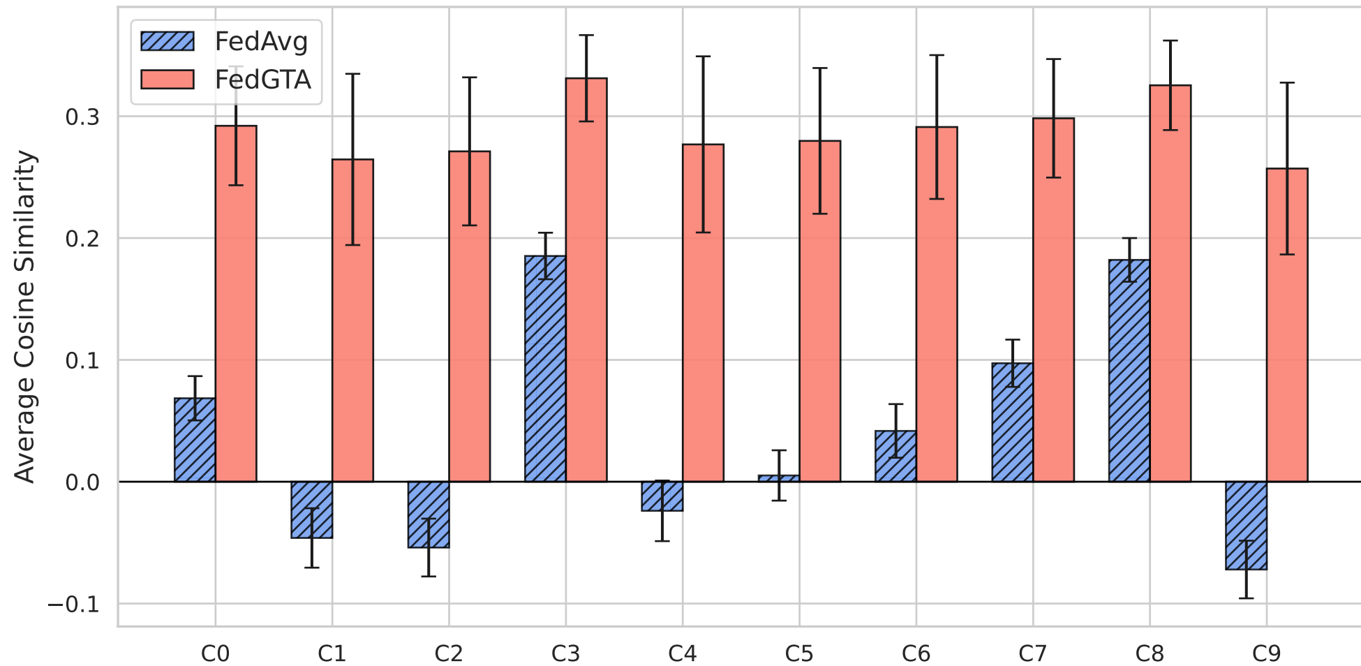
Client-wise Cosine Similarity Distribution - ImageNet ( \alpha=0.01 )
