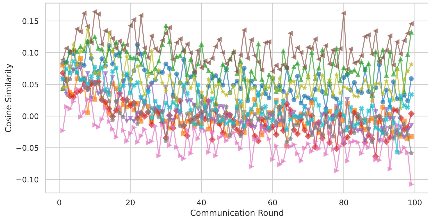
FedAvg - Client Cosine Similarity [ImageNet \alpha=0.1 ]
