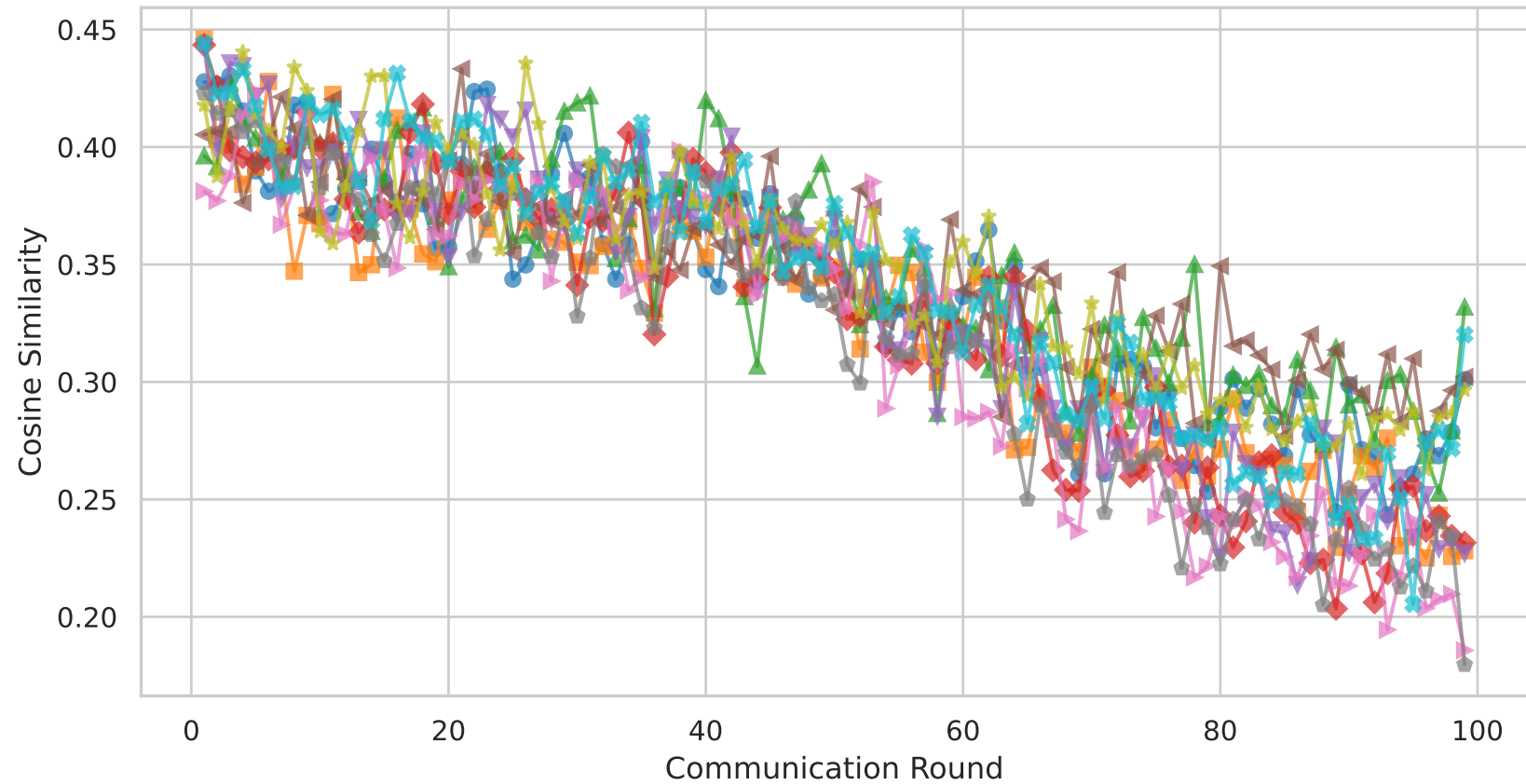
FedGTA - Client Cosine Similarity [ImageNet \alpha=0.1 ]
