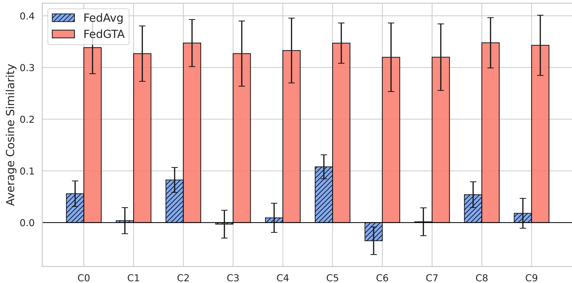
Client-wise Cosine Similarity Distribution - ImageNet ( \alpha=0.1 )
