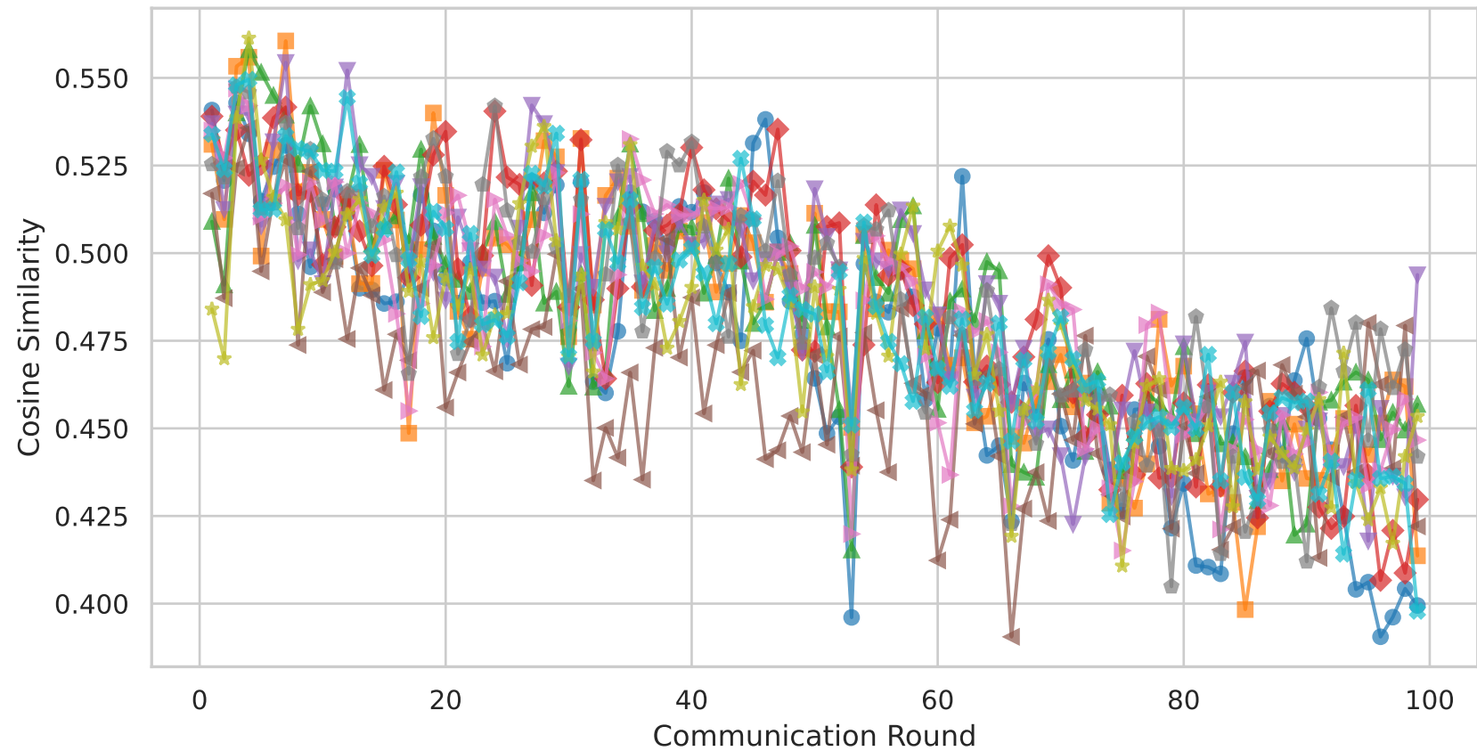
FedGTA - Client Cosine Similarity [ImageNet \alpha=1 ]
