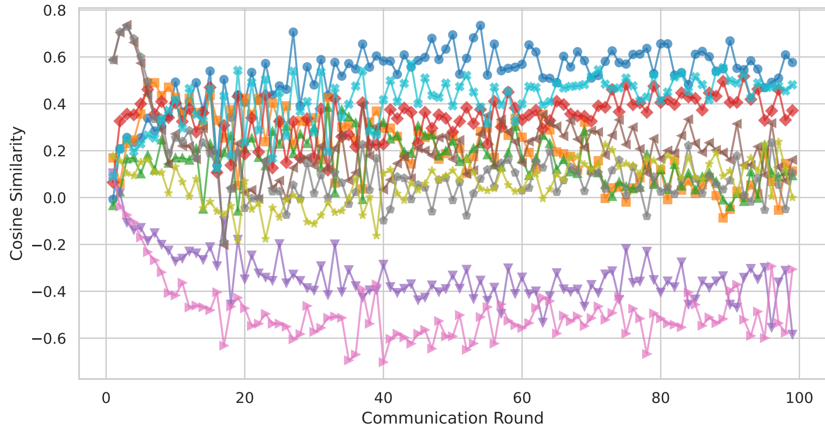
FedAvg - Client Cosine Similarity [MNIST \alpha=0.01 ]
