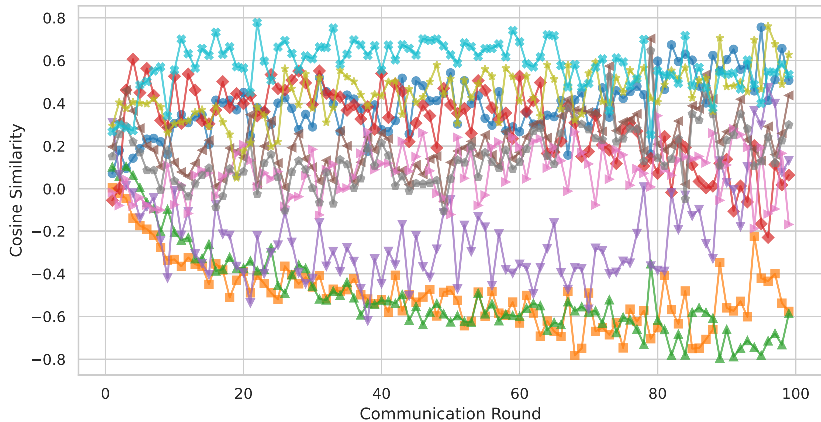
FedAvg - Client Cosine Similarity [MNIST \alpha=0.1 ]
