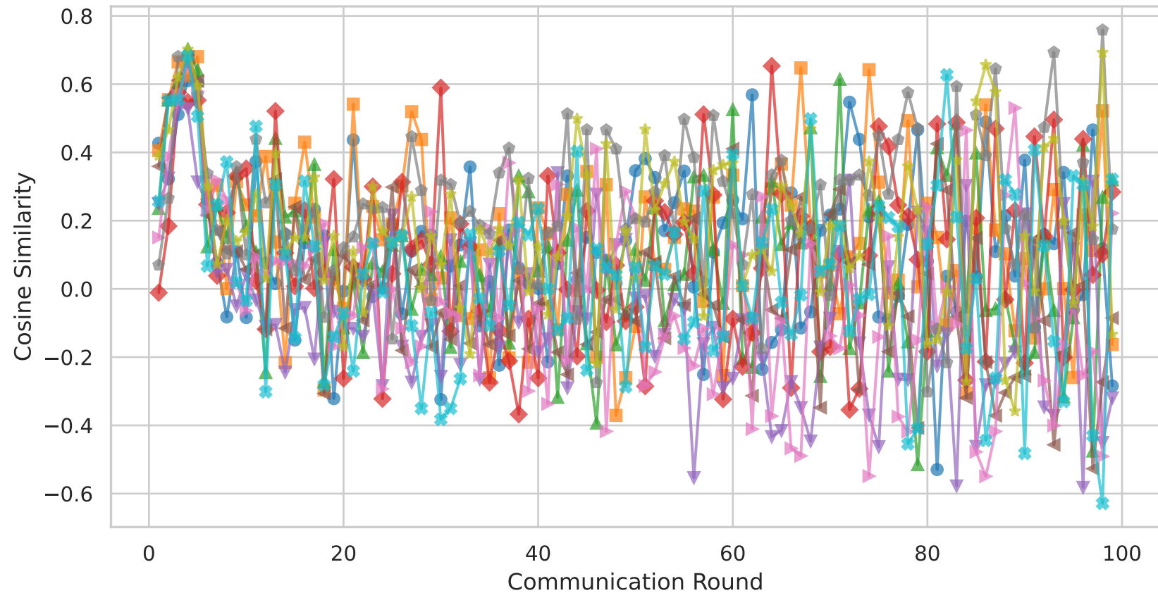
FedAvg - Client Cosine Similarity [MNIST \alpha=1 ]
