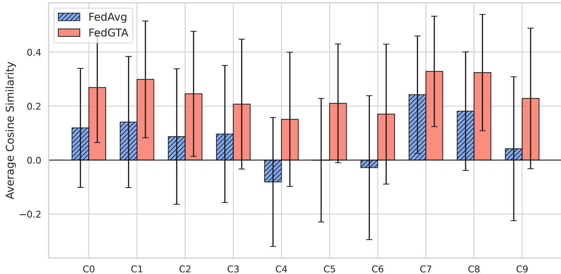
Client-wise Cosine Similarity Distribution - MNIST ( \alpha=1 )
