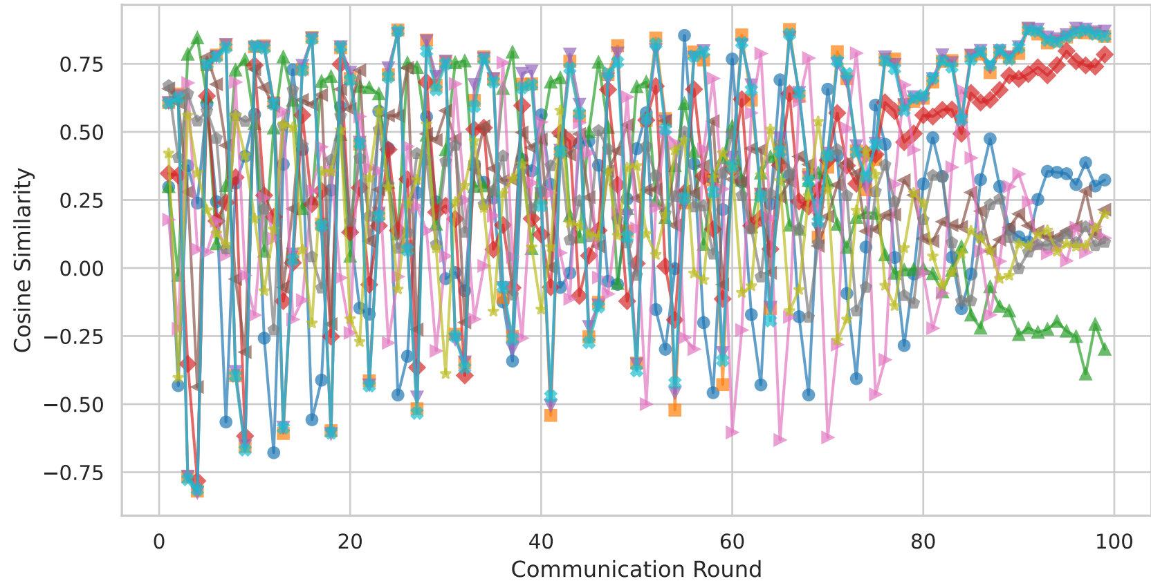
FedGTA - Client Cosine Similarity [CIFAR10 \alpha=0.01 ]
