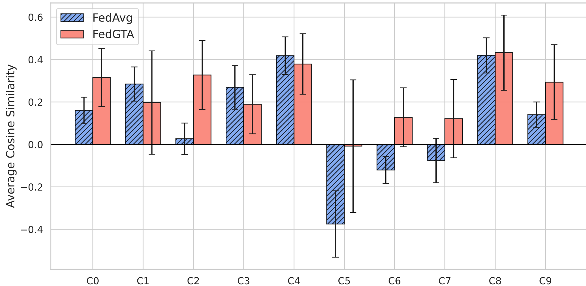
Client-wise Cosine Similarity Distribution - CIFAR10 ( \alpha=0.1 )
