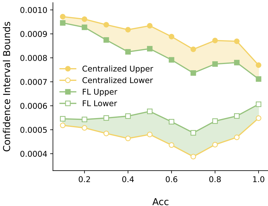
Diabetes-bmi ( \alpha_{Dir} = 0.01 ) (Fixed \lambda = 0.3 )
