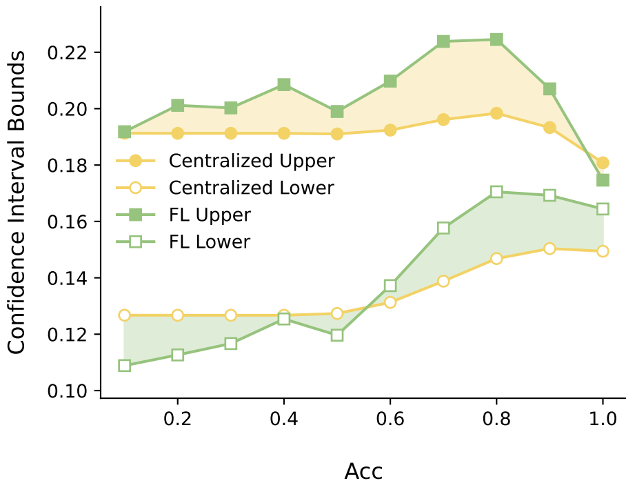
Diabetes-hypertension ( \alpha_{Dir} = 0.01 ) (Fixed \lambda = 0.3 )
