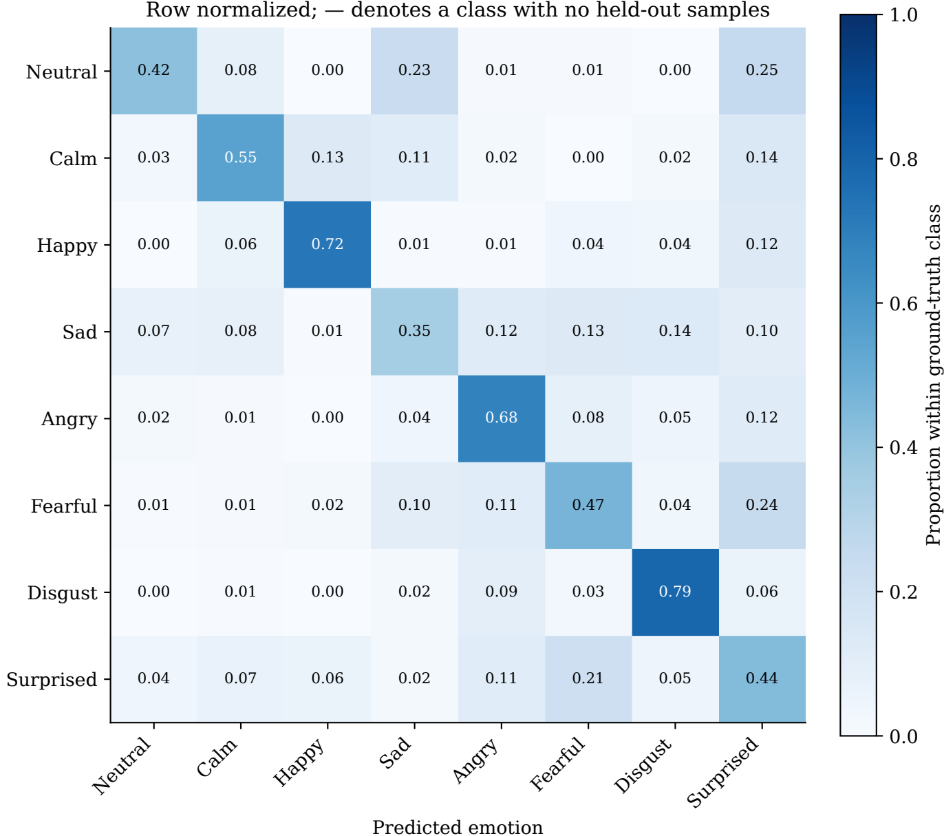
Adapted Intermediate Attention — pooled held-out predictions | 6/6 folds Row normalized; — denotes a class with no held-out samples
