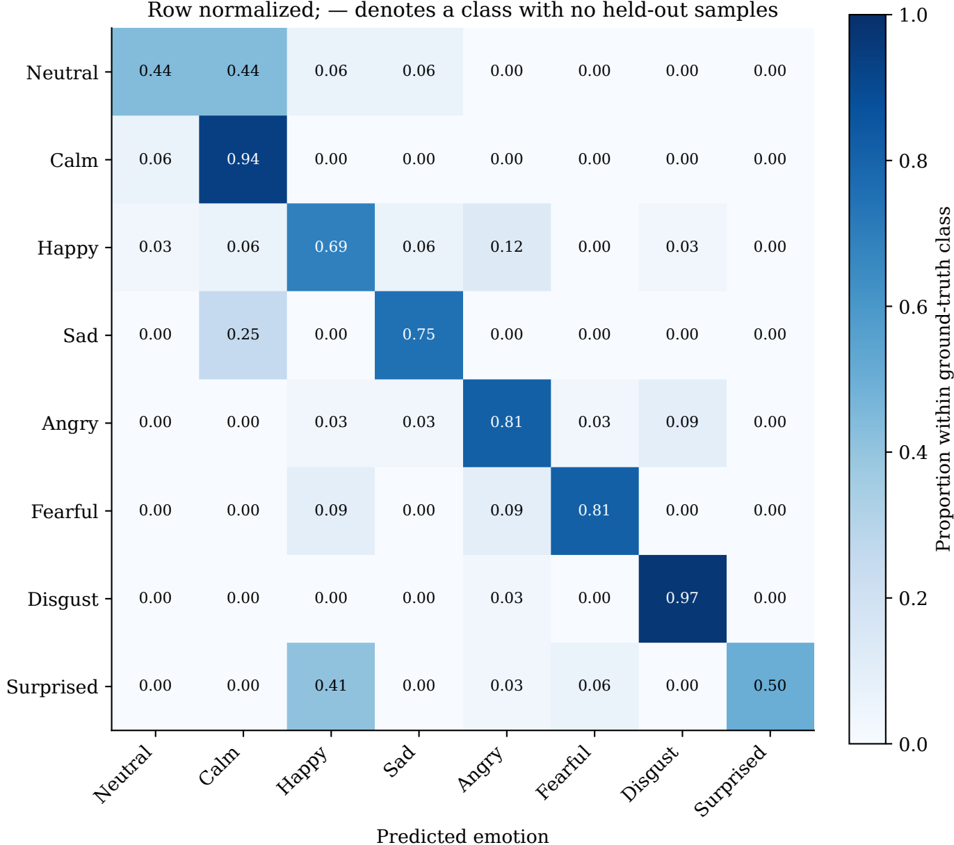
Audio — Fold 2 | 6/6 folds Row normalized; — denotes a class with no held-out samples
