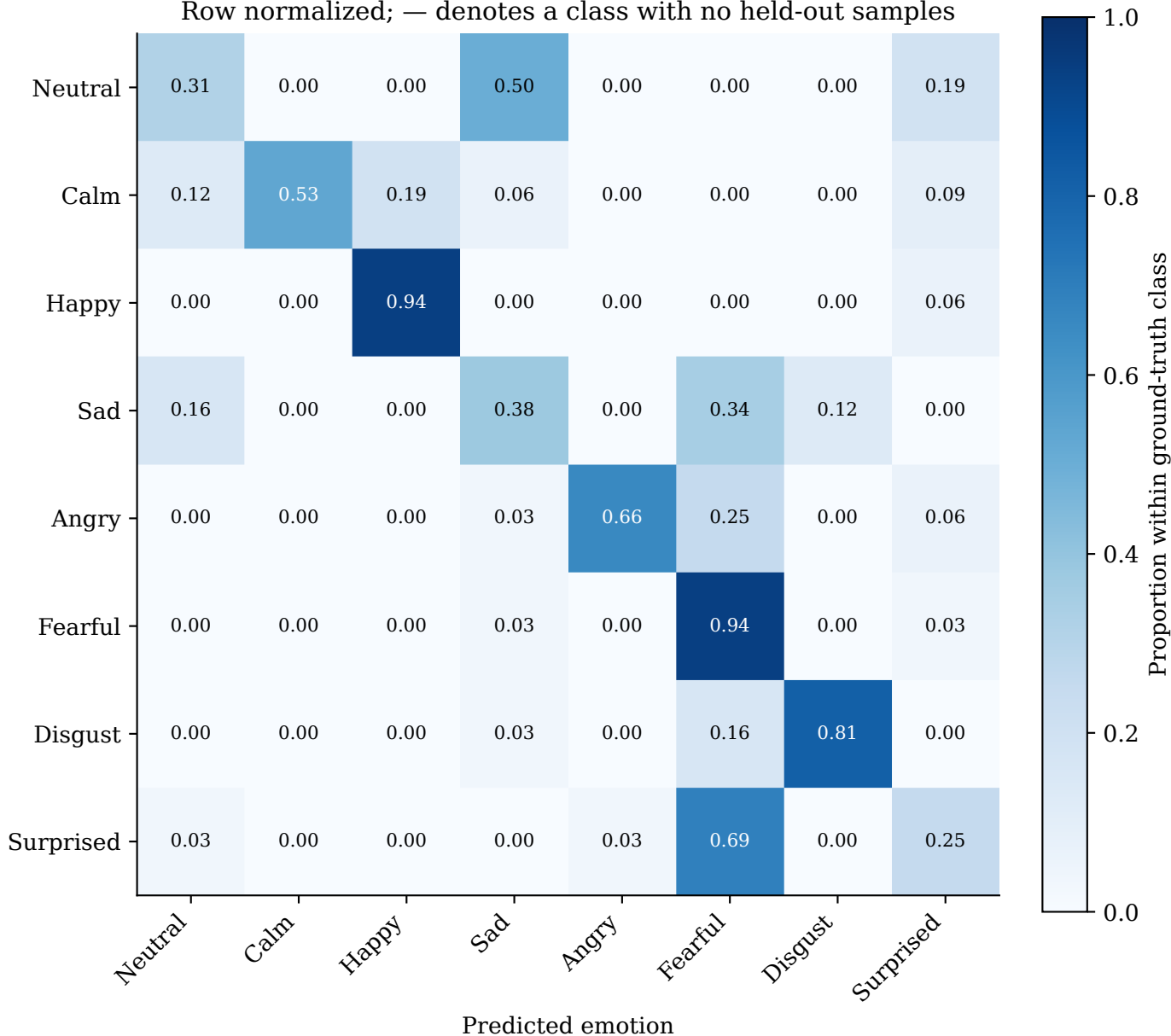
Adapted Intermediate Attention — Fold 2 | 6/6 folds Row normalized; — denotes a class with no held-out samples
