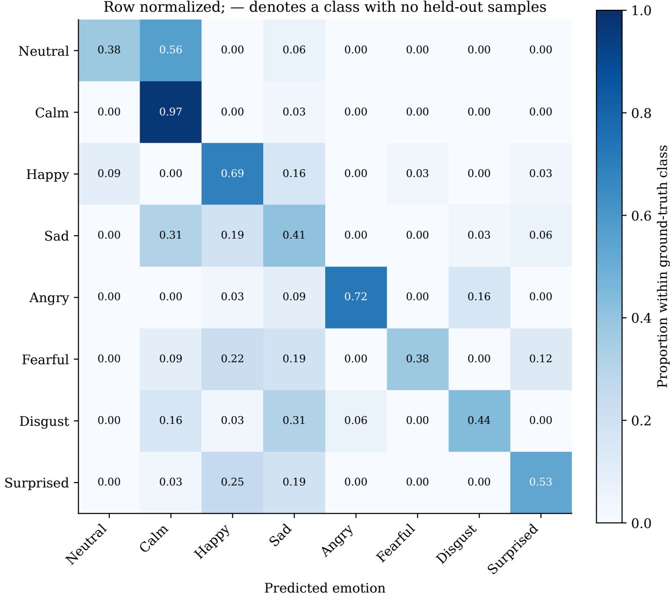
Audio — Fold 3 | 6/6 folds Row normalized; — denotes a class with no held-out samples
