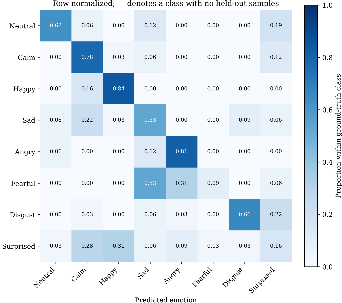
Adapted Intermediate Attention — Fold 4 | 6/6 folds Row normalized; — denotes a class with no held-out samples
