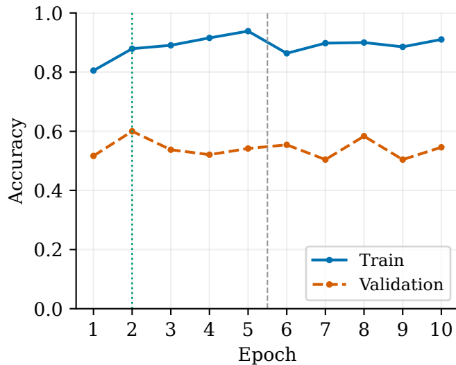
Adapted Intermediate Attention — Fold 4 | 6/6 folds Dotted green: best validation epoch; dashed gray: training stage change
