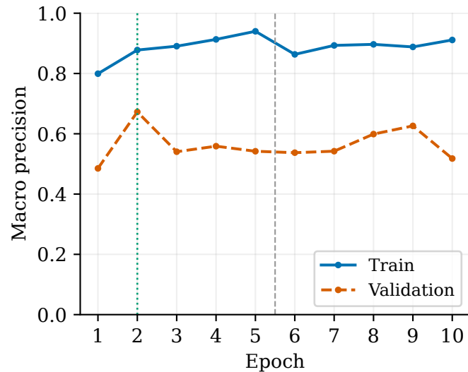
Adapted Intermediate Attention — Fold 4 | 6/6 folds Dotted green: best validation epoch; dashed gray: training stage change
