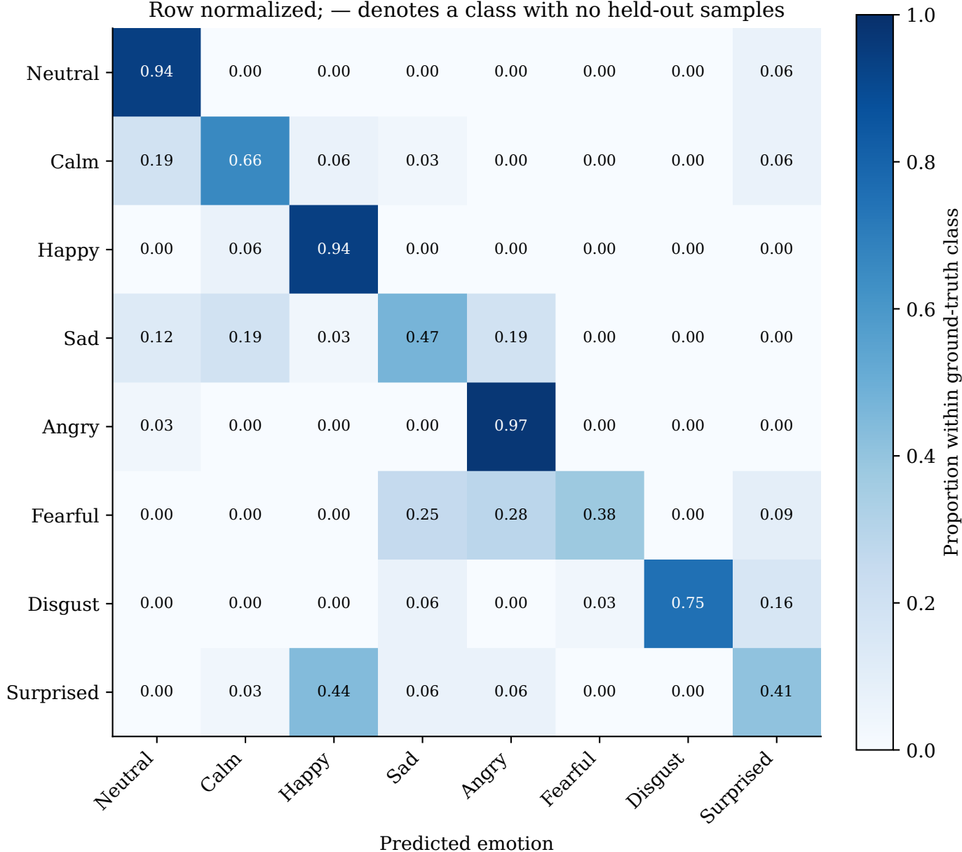
Gated fusion — Fold 4 | 6/6 folds Row normalized; — denotes a class with no held-out samples
