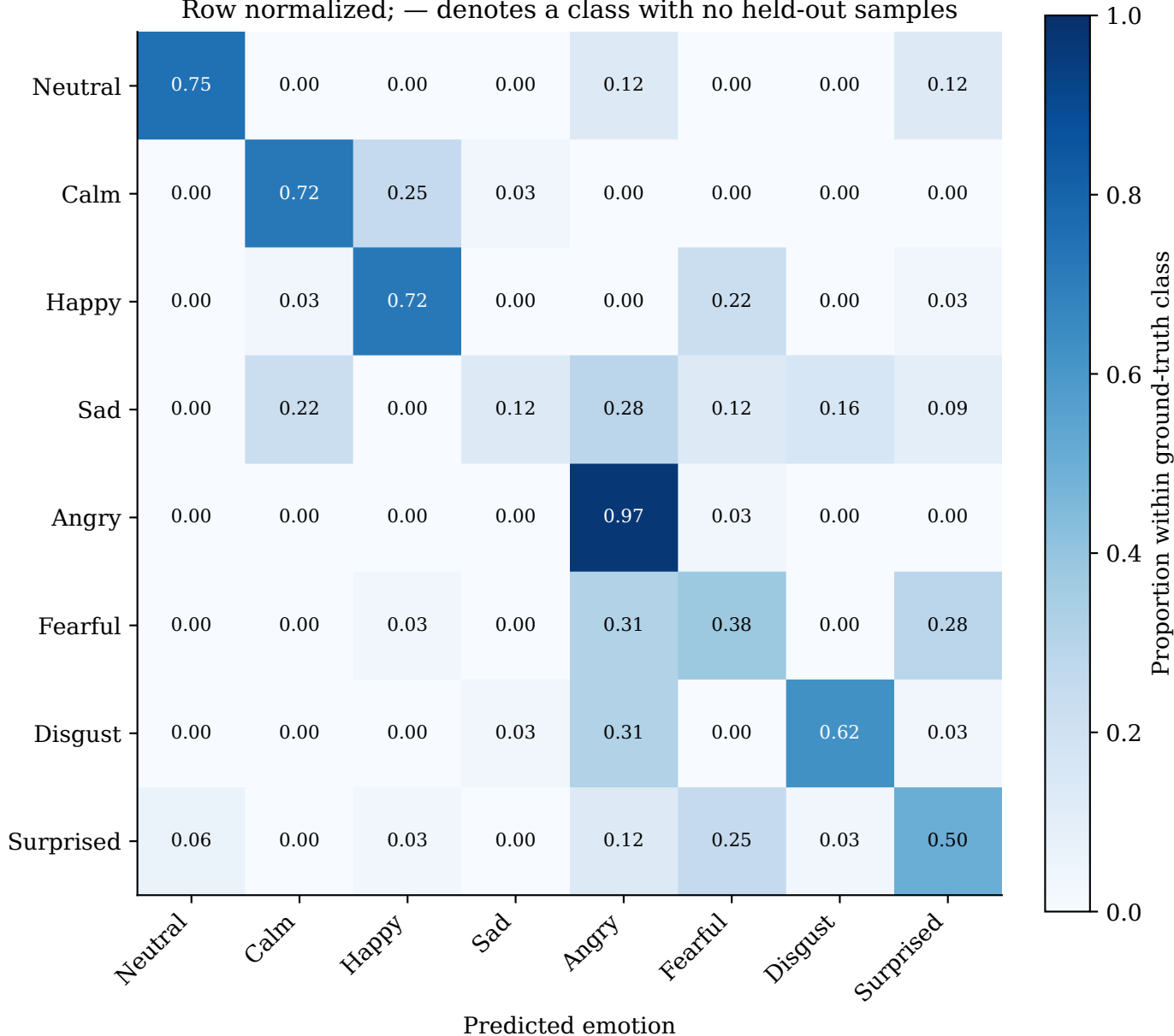
Cross-attention — Fold 6 | 6/6 folds Row normalized; — denotes a class with no held-out samples
