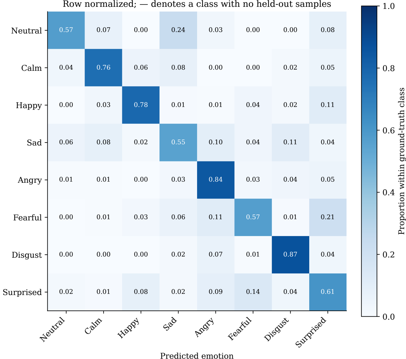
Gated fusion — pooled held-out predictions | 6/6 folds Row normalized; — denotes a class with no held-out samples
