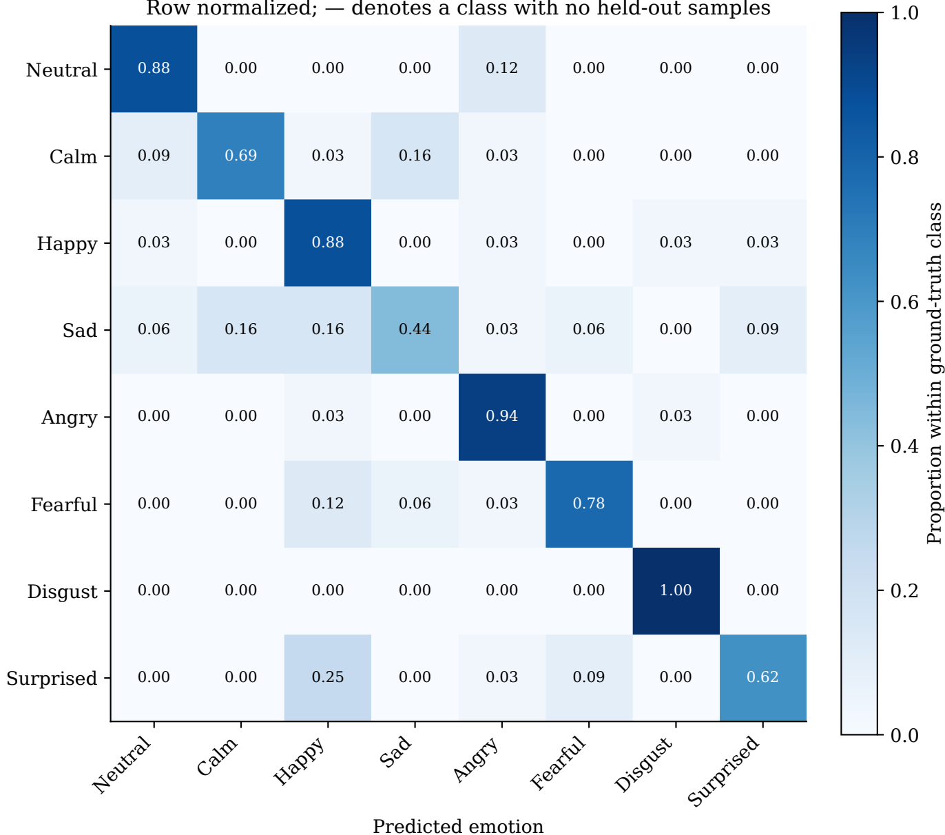
Audio — Fold 1 | 6/6 folds Row normalized; — denotes a class with no held-out samples
